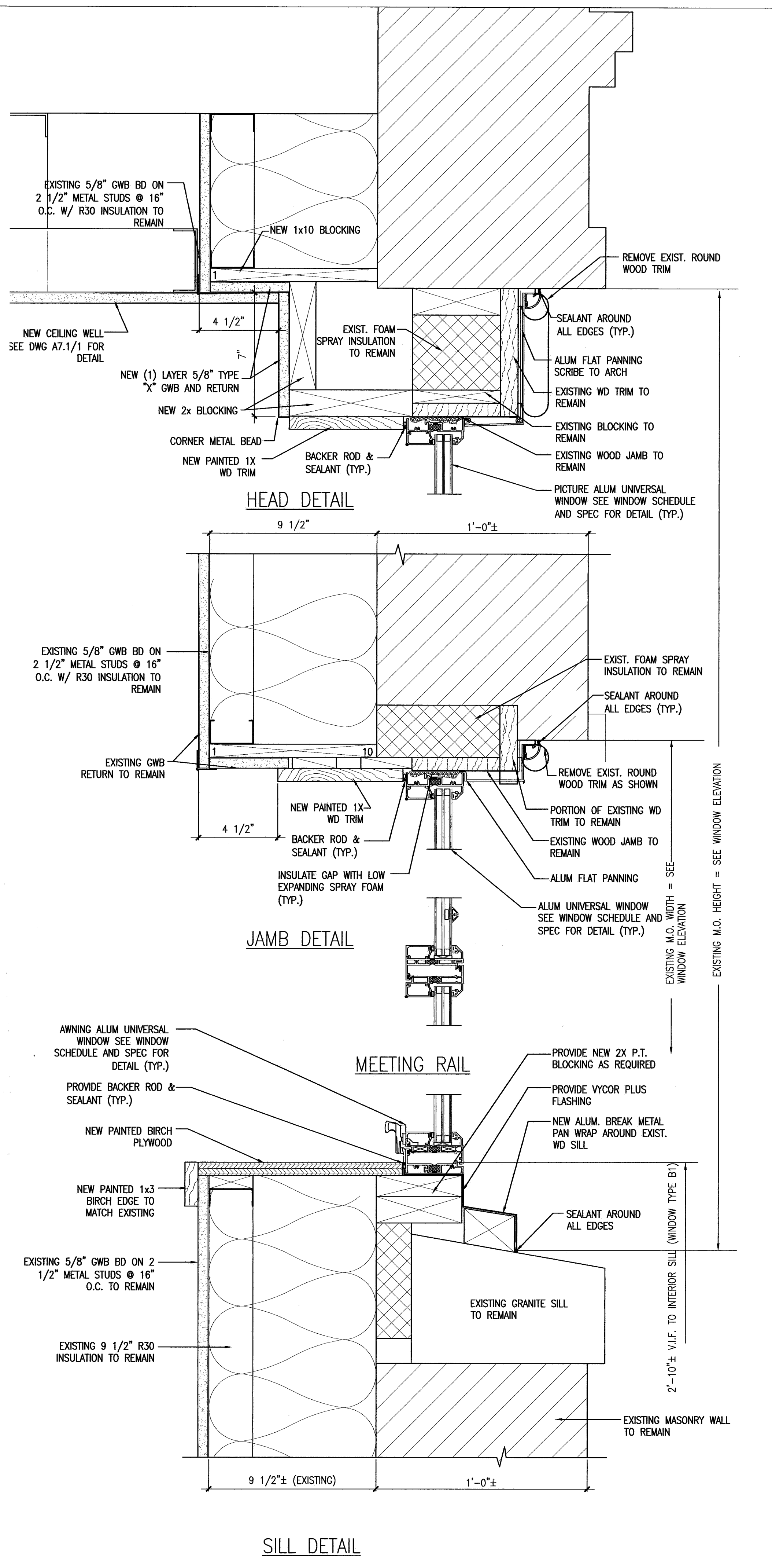
3 NEW WINDOW SILL, JAMB AND HEAD DETAILS @ AWNING/ FIXED UNIT REFERENCED FROM: SCALE: 3" = 1'-0"
