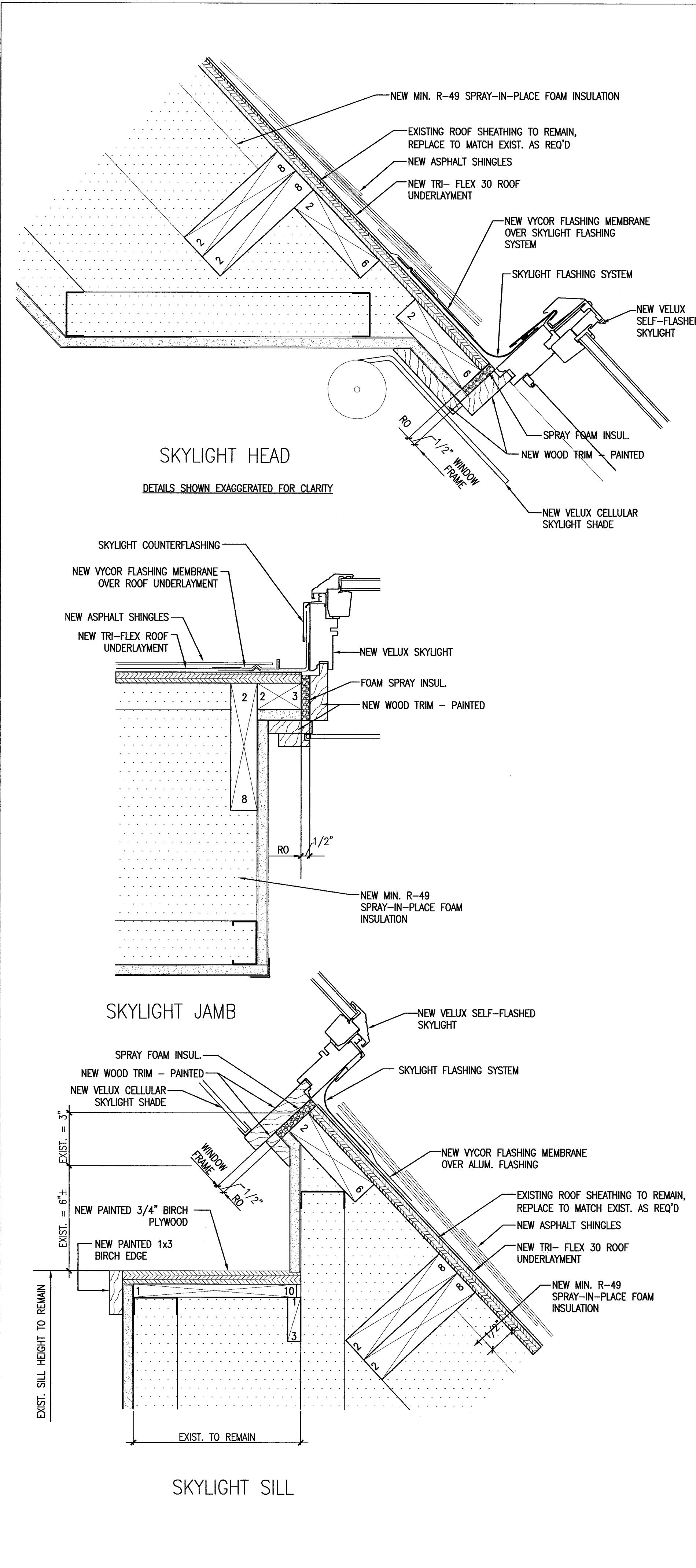
1 SKYLIGHT DETAILS REFERENCED FROM: SCALE: 3" = 1'-0"
