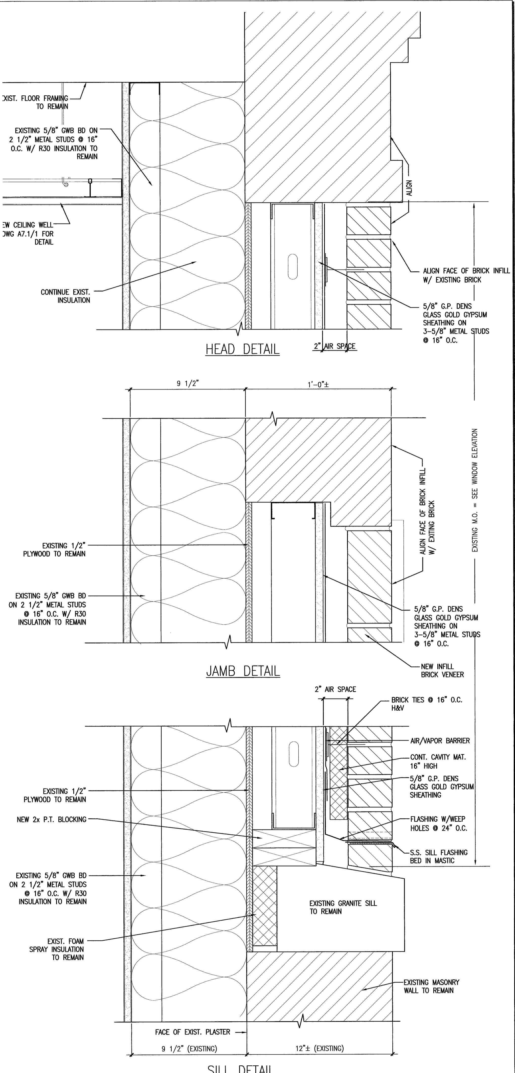
3 NEW INFILL BRICK VENEER - SILL, JAMB AND HEAD DETAILS REFERENCED FROM: SCALE: 5" = 1'-0"
