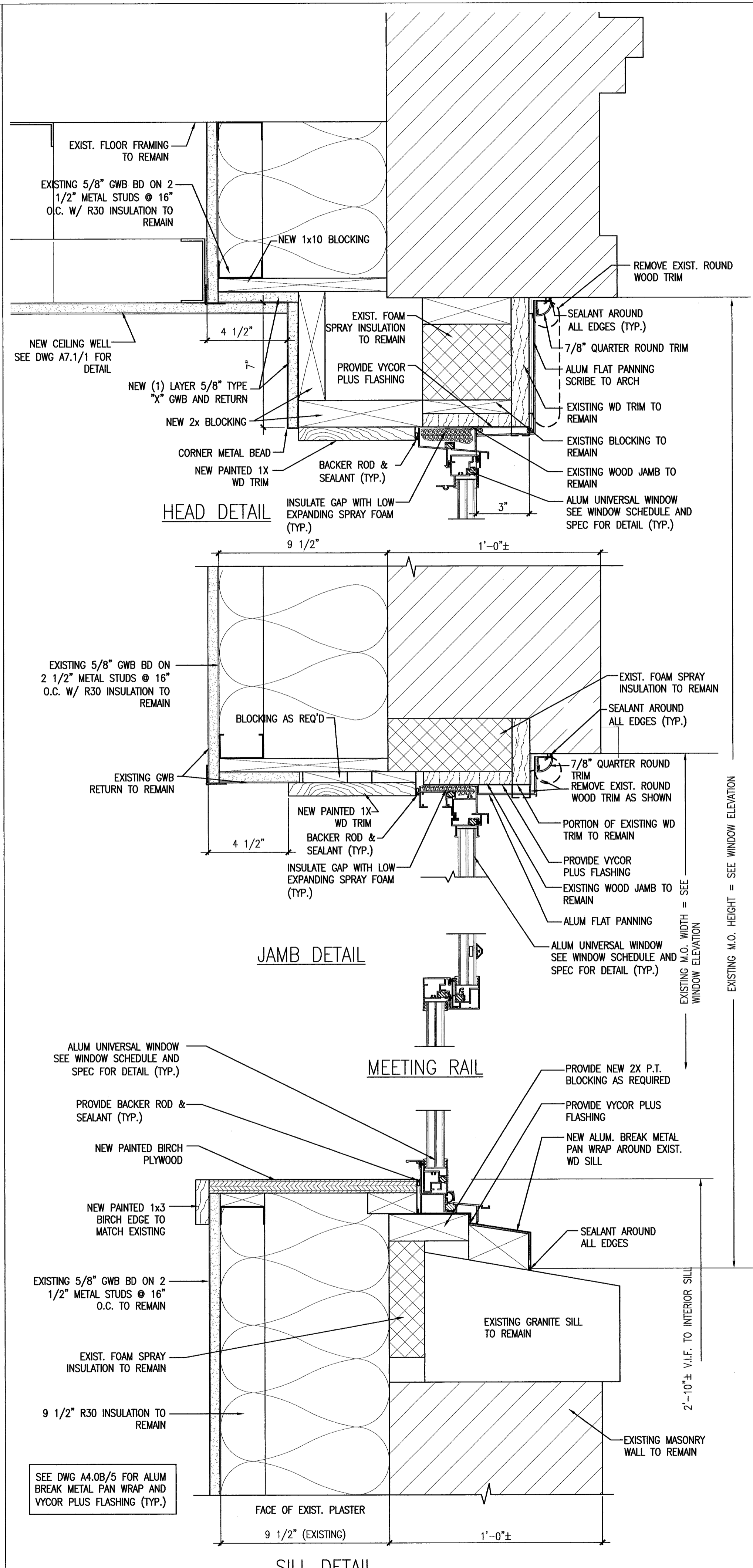
2 NEW WINDOW - SILL, JAMB AND HEAD DETAILS REFERENCED FROM: SCALE: 5" = 1'-0"
