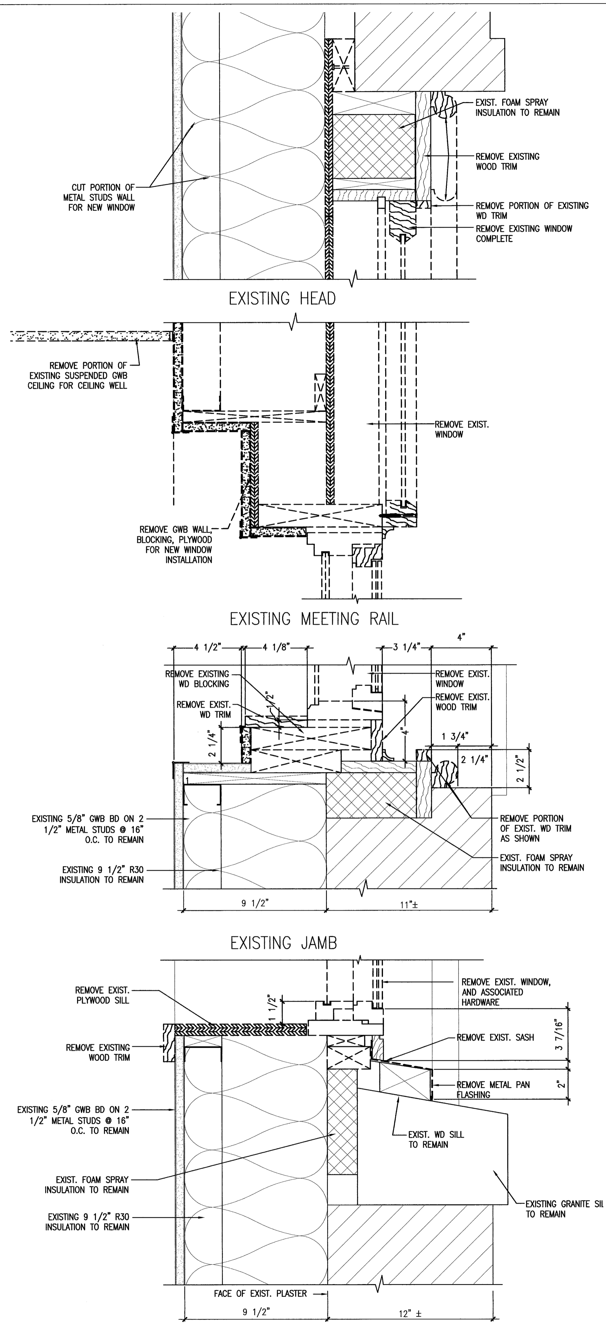
1 EXISTING WINDOW - SILL, JAMB AND HEAD DETAILS REFERENCED FROM: SCALE: 5" = 1'-0"
