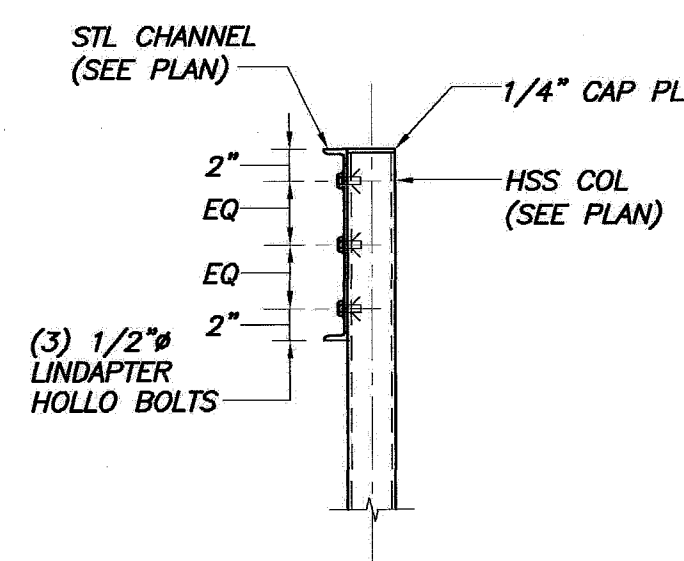
SECTION 6 1"=1'-0" S1.2
