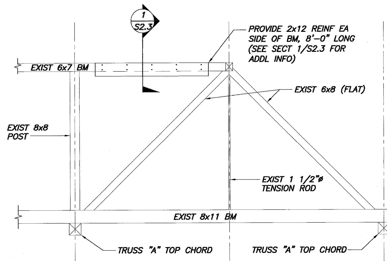
ROOF TRUSS ELEVATION A-A 1/4"=1'-0"
