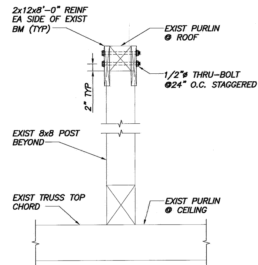
SECTION 1 3/4"=1'-0" S2.3
