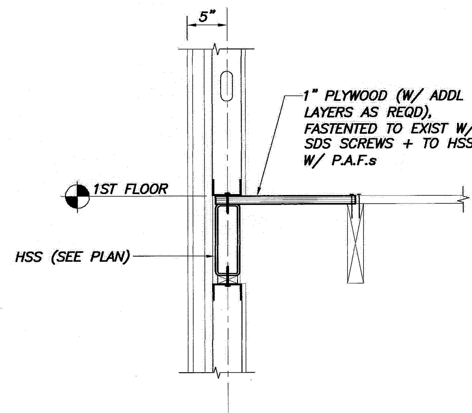
SECTION 4 1"=1'-0" S1.2
