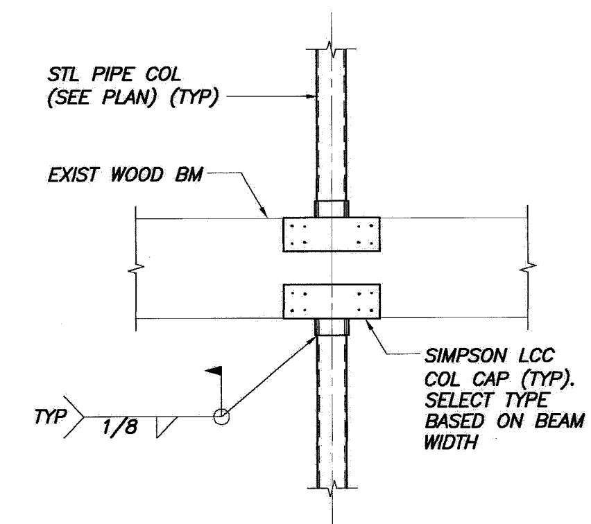
SECTION 3 3/4"=1'-0" S1.3
