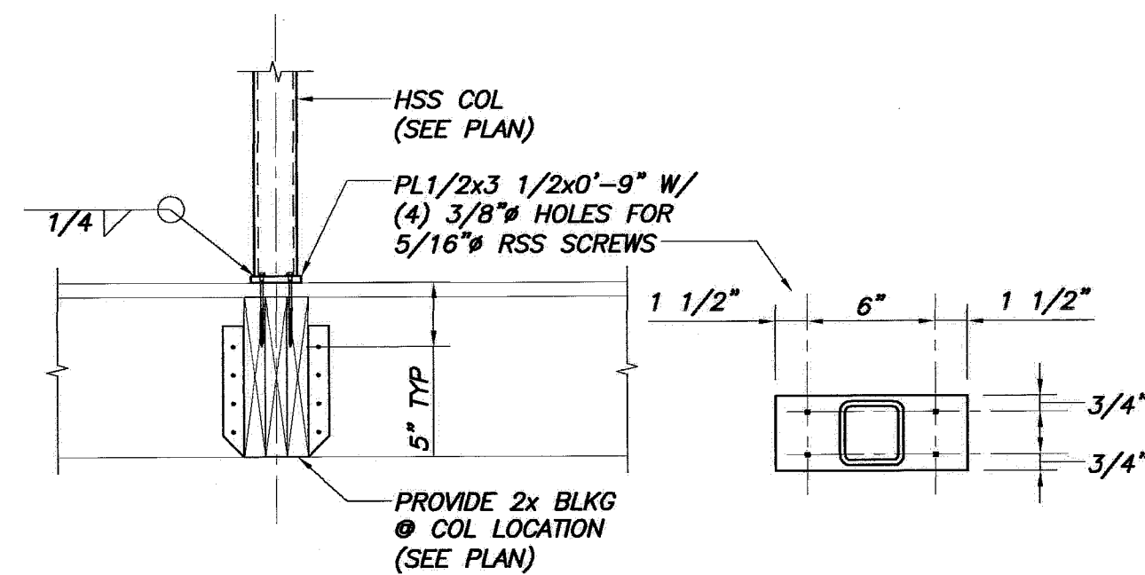
SECTION 5 1"=1'-0" S1.2
