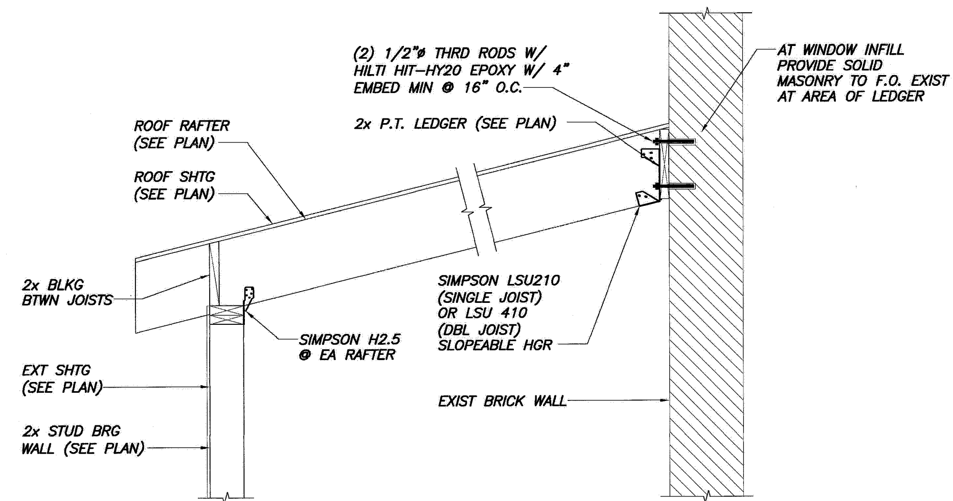
SECTION 2 3/4"=1'-0" S1.3
