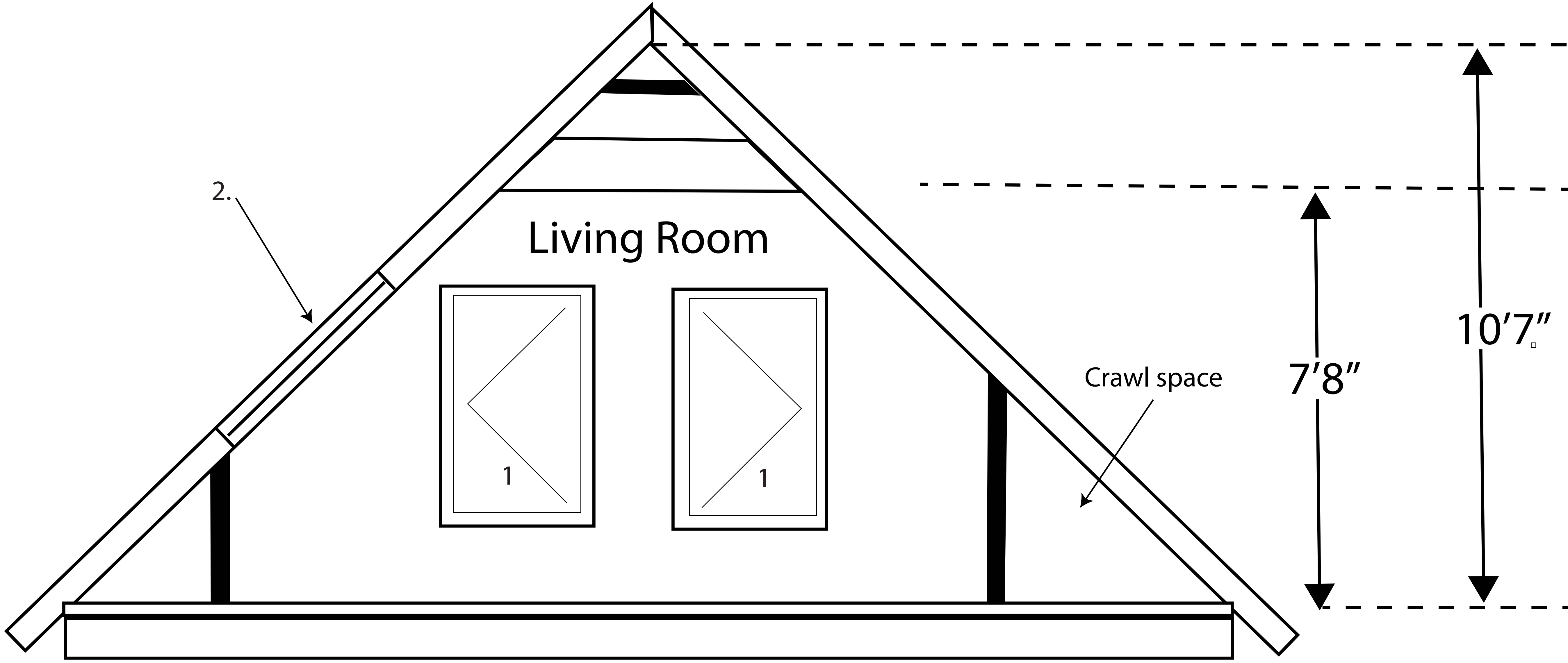
A 3.1 Gable
