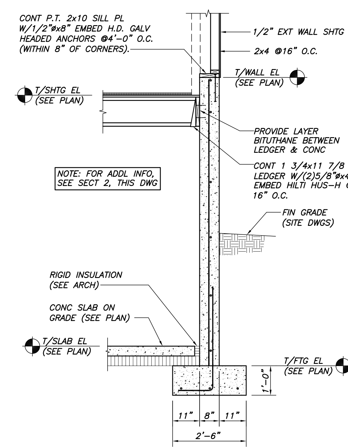
SECTION 3 1/2"=1'-0"
