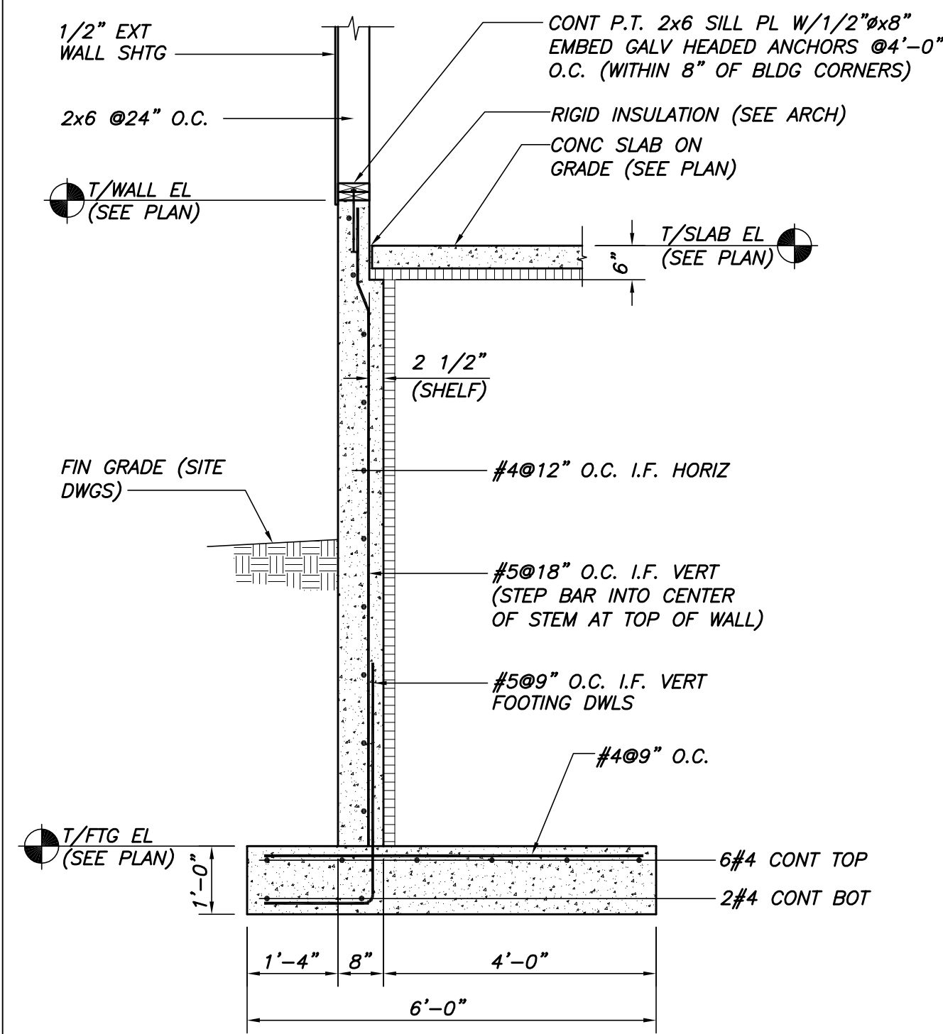
SECTION 1 1/2"=1'-0"
