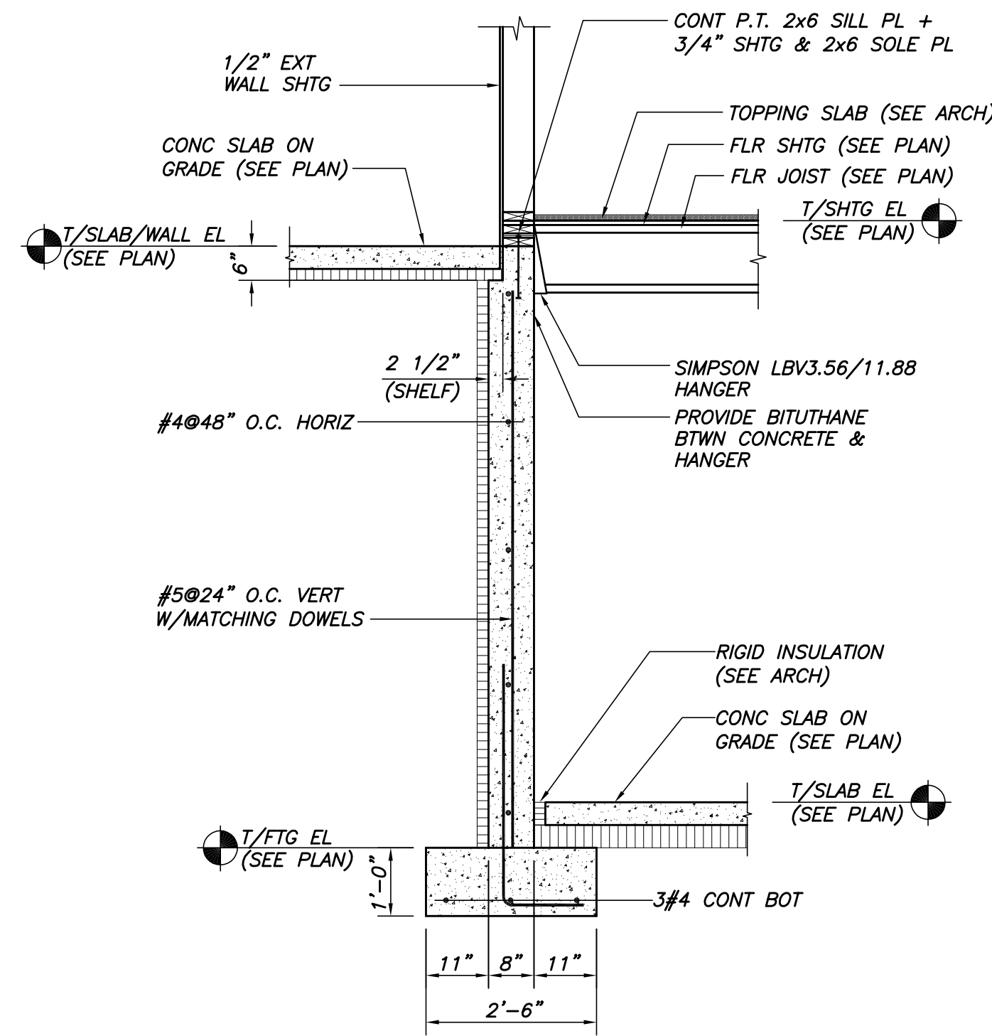
SECTION 2 1/2"=1'-0"
