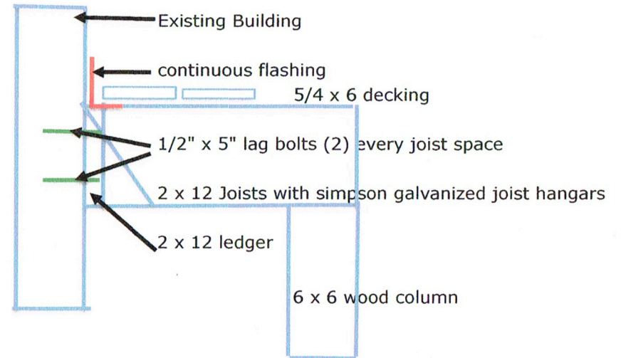
Ledger Detail. Typ.
