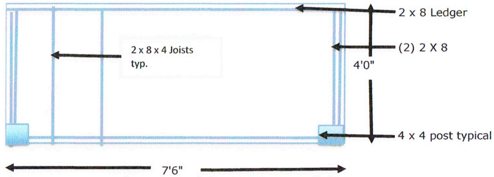
Third floor deck plan
