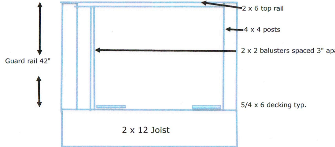
Guard Rail
