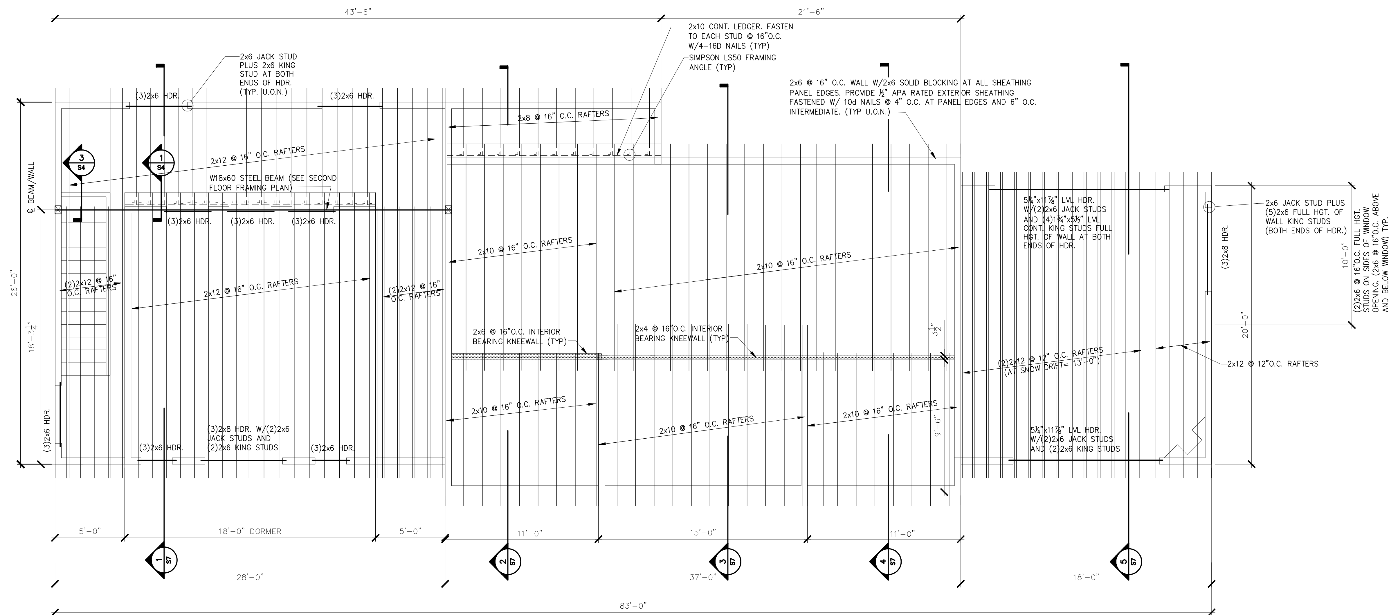
ROOF FRAMING PLAN 1/4" = 1'-0"
