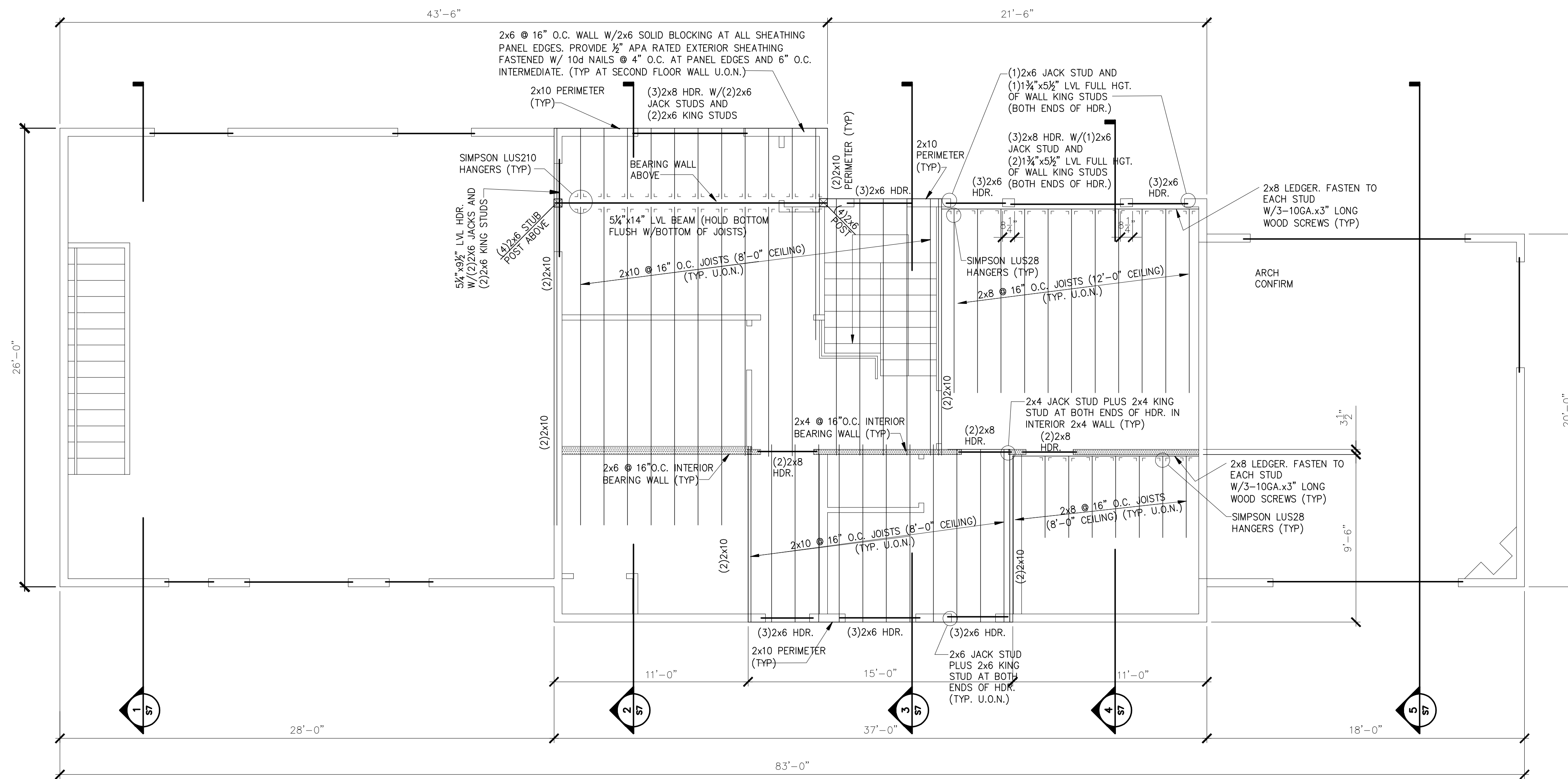
ATTIC FLOOR FRAMING PLAN 1/4" = 1'-0"
