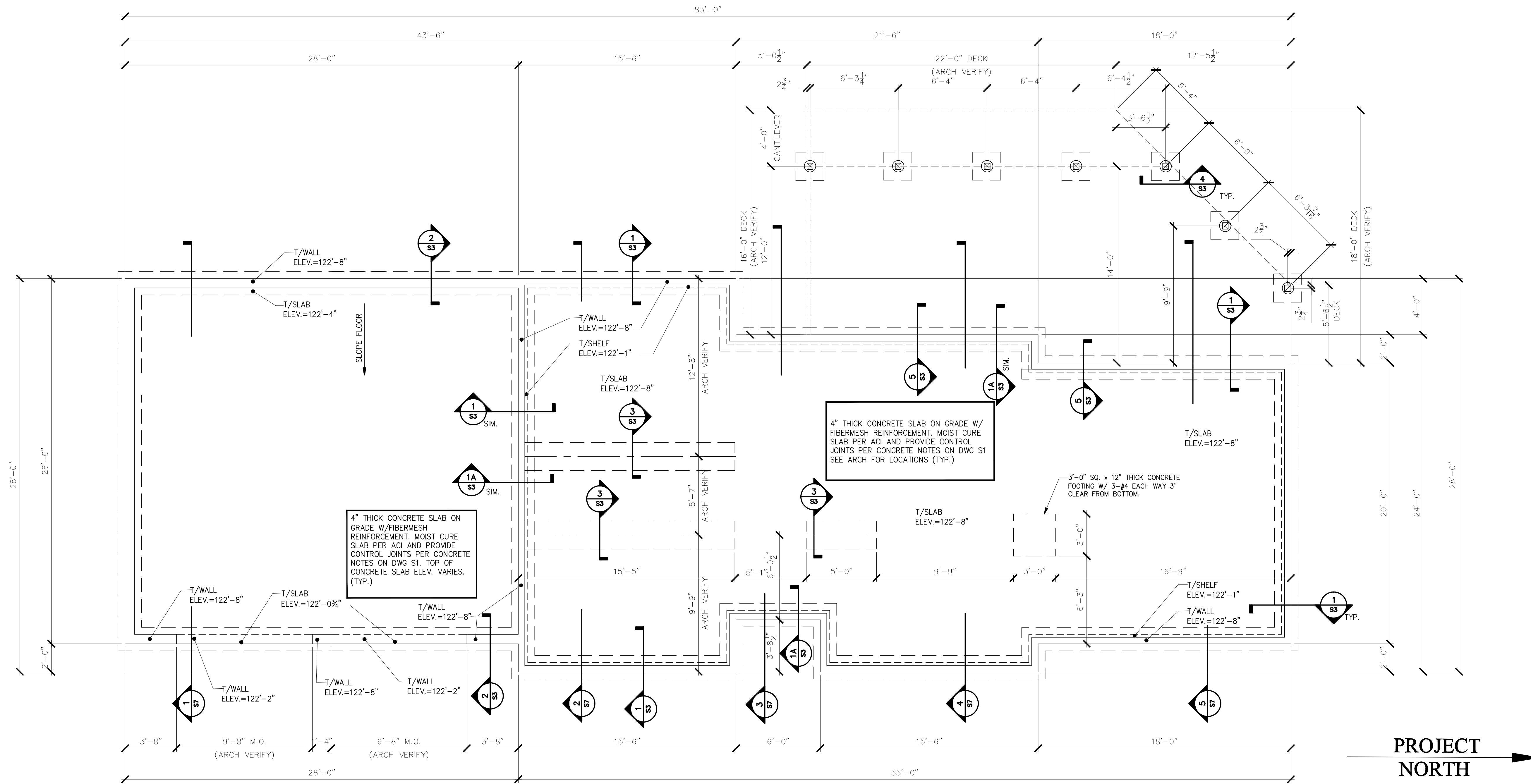
FOUNDATION PLAN 1/4" = 1'-0"
