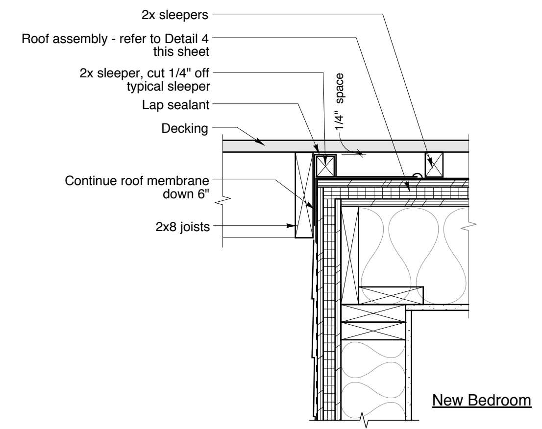
6 Detail at Deck/Ext Wall SCALE: 1 1/2" = 1'-0"
