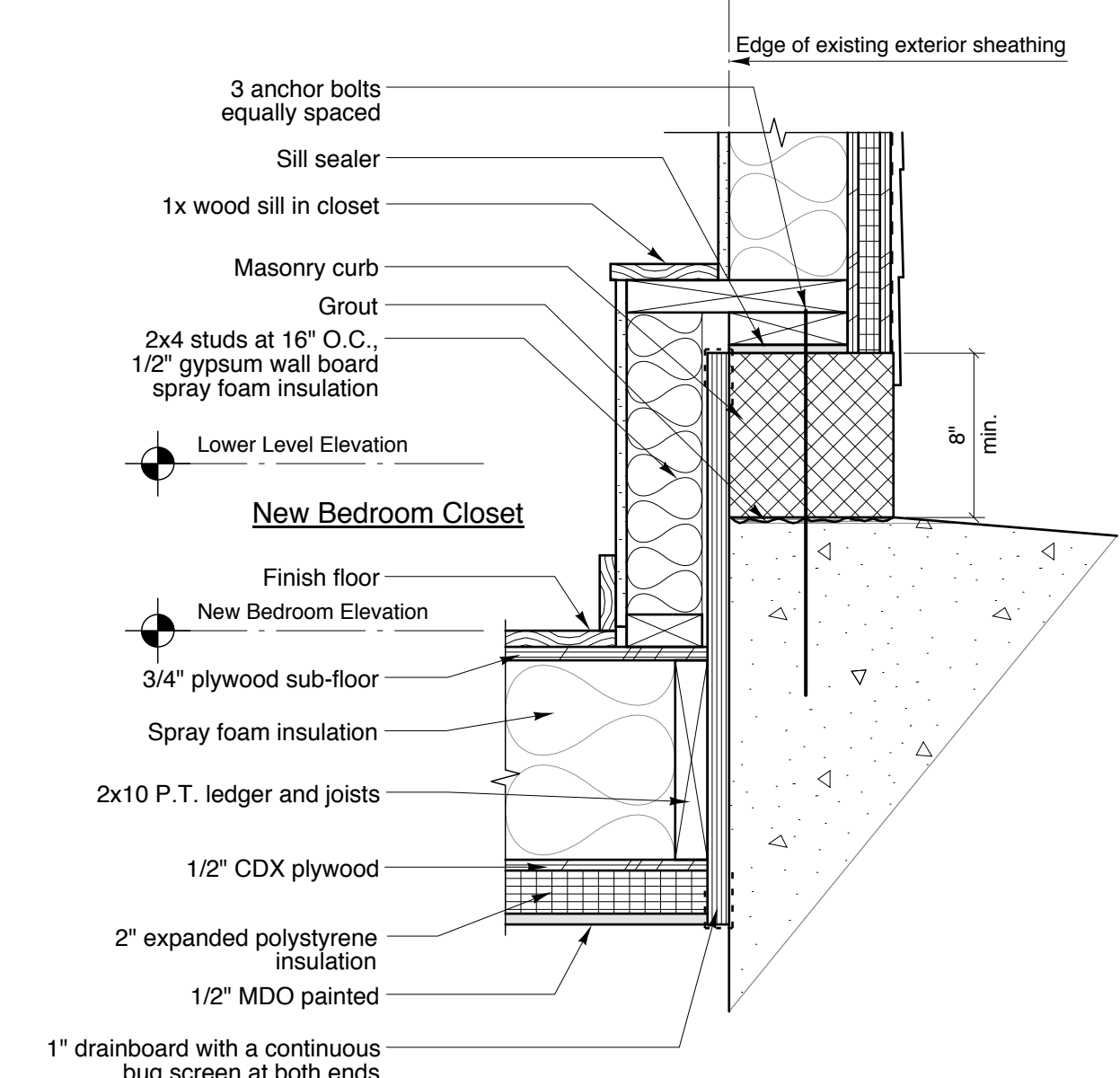
3 Detail at Floor/Exist Conc. Wall SCALE: 1 1/2" = 1'-0"
