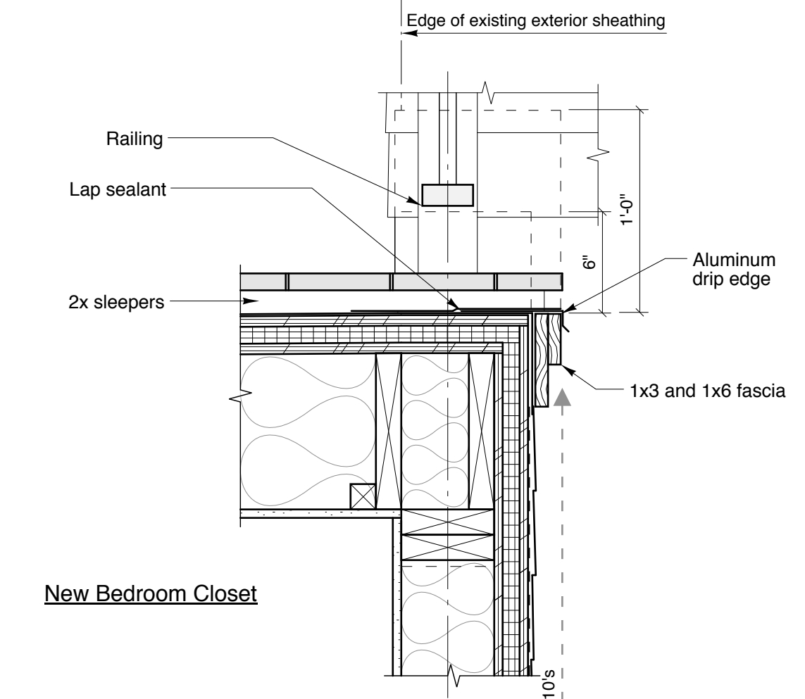
1 Ceiling and Deck Details SCALE: 1 1/2" = 1'-0"
