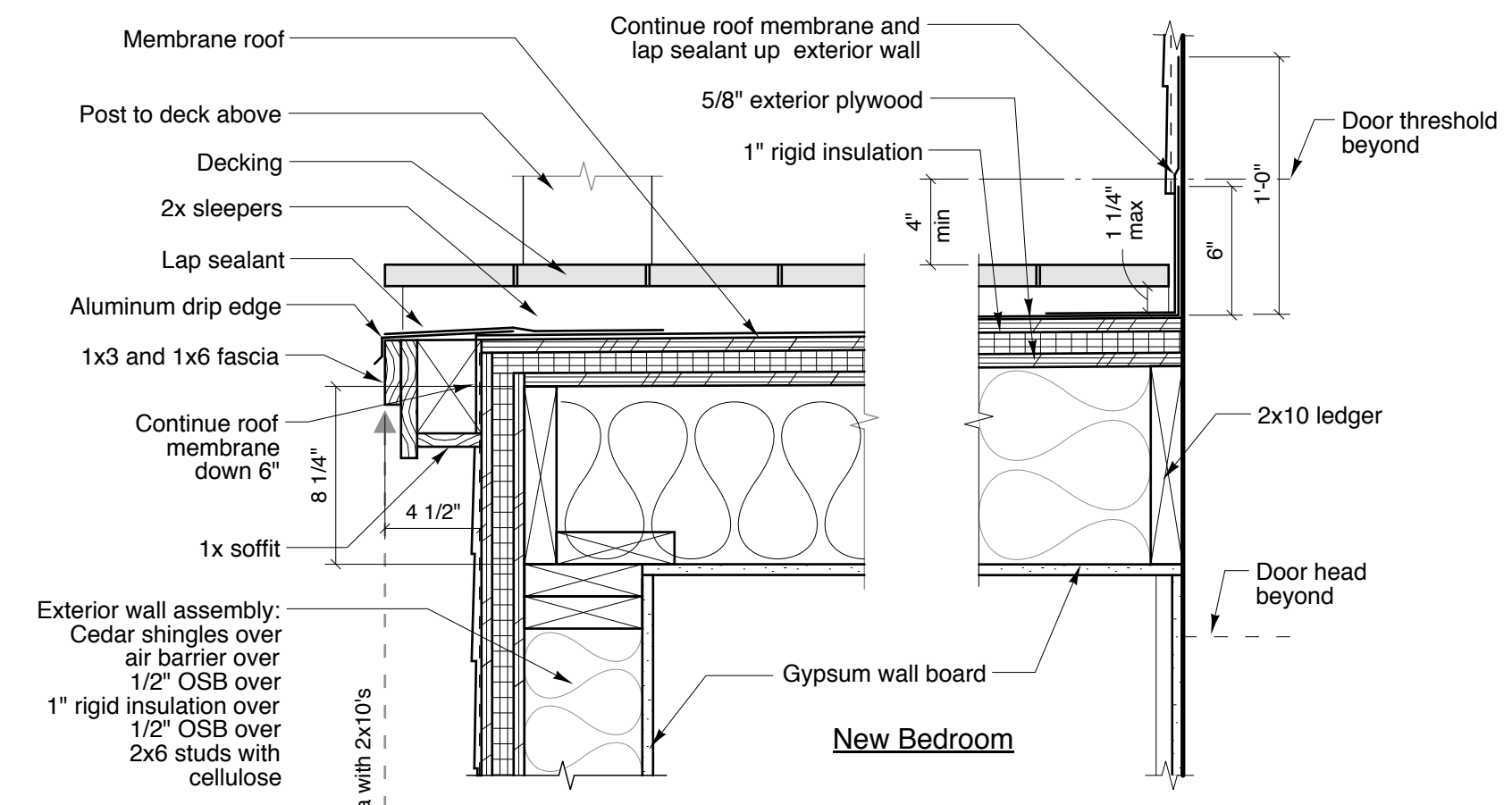
4 Ceiling and Deck Details SCALE: 1 1/2" = 1'-0"
