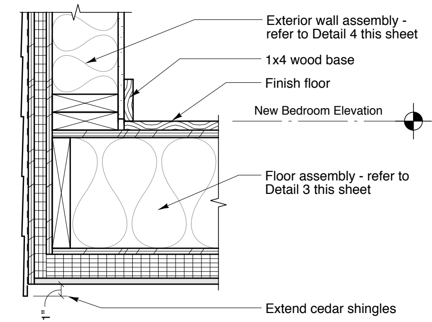
7 Detail at Ext. Wall/Floor SCALE: 1 1/2" = 1'-0"
