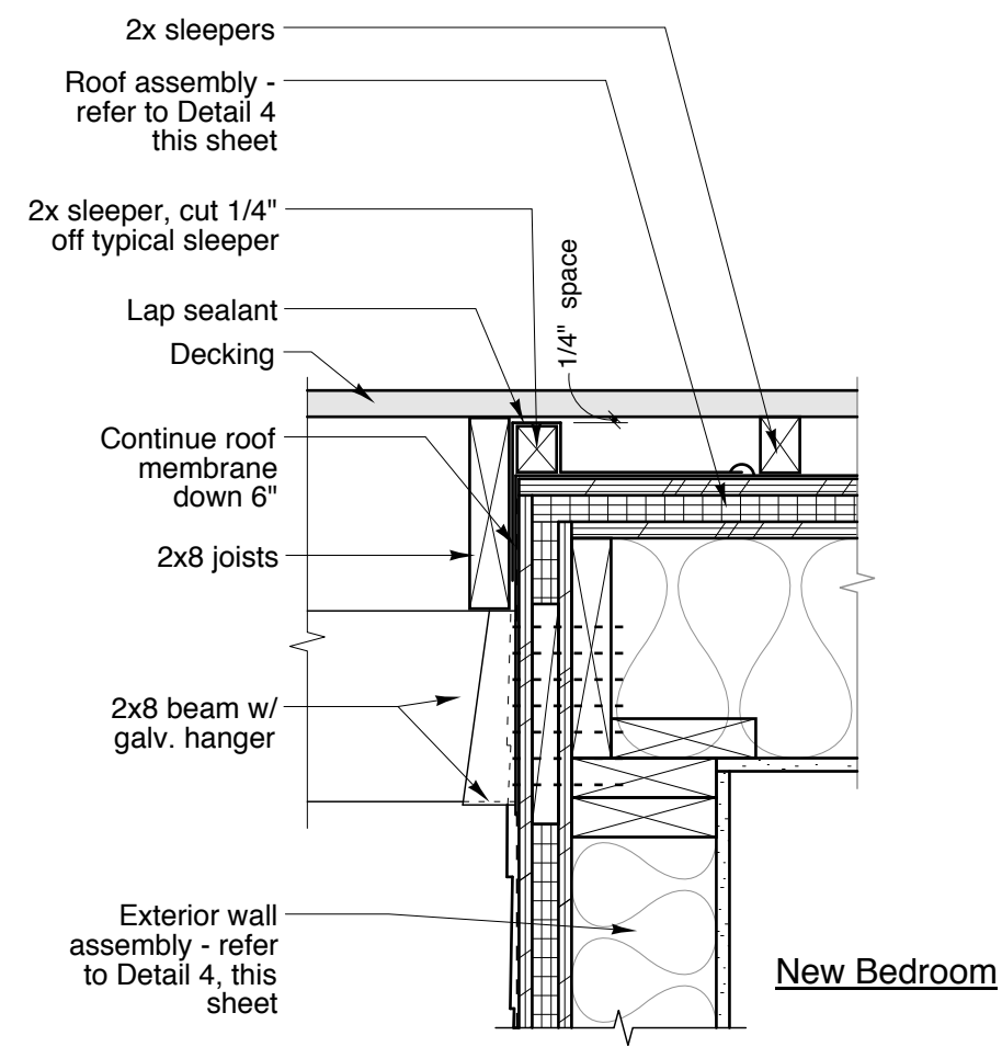
8 Detail at Beam Connection SCALE: 1 1/2" = 1'-0"
