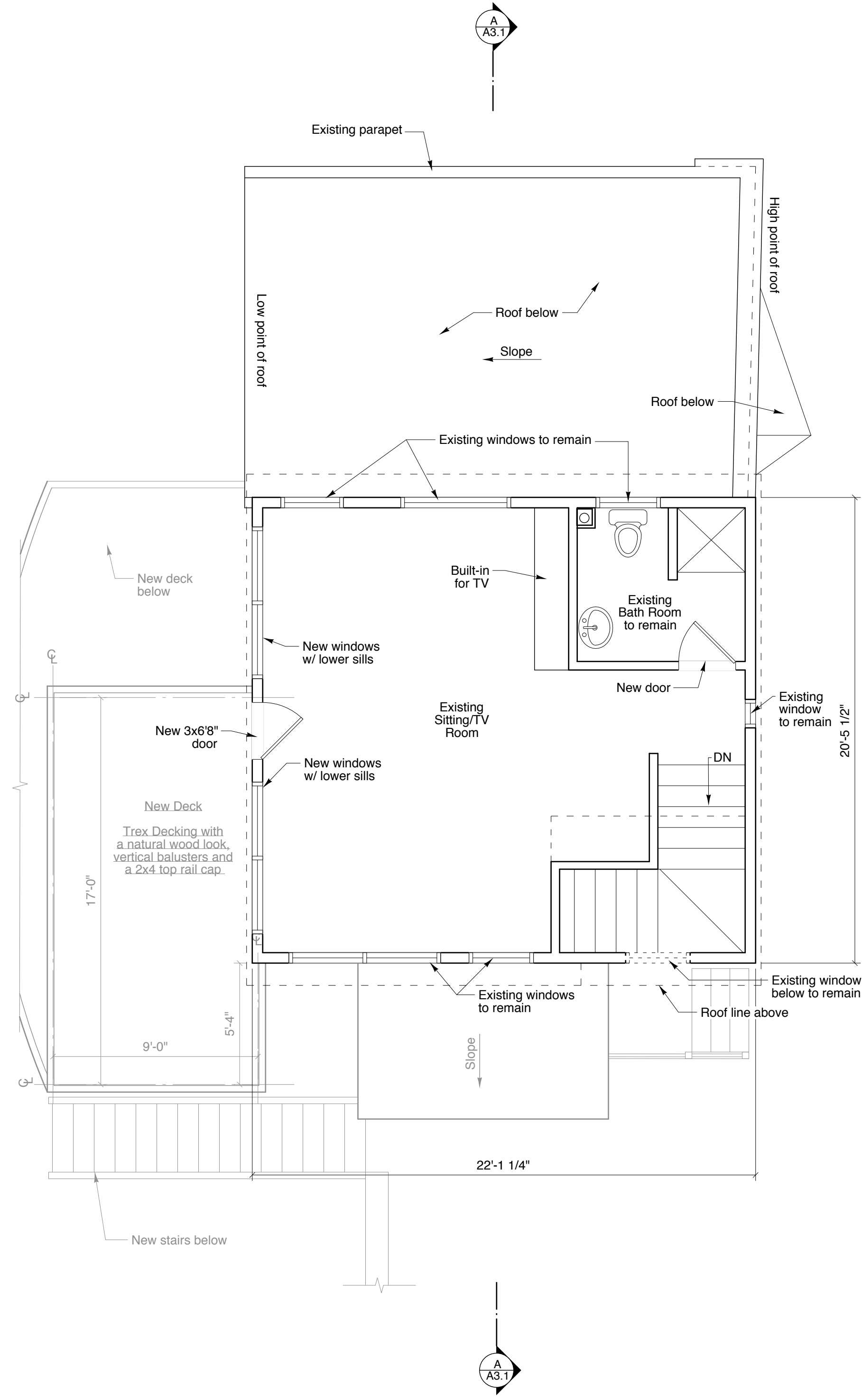
3 Upper Level Floor Plan SCALE: 1/4" = 1'-0"
