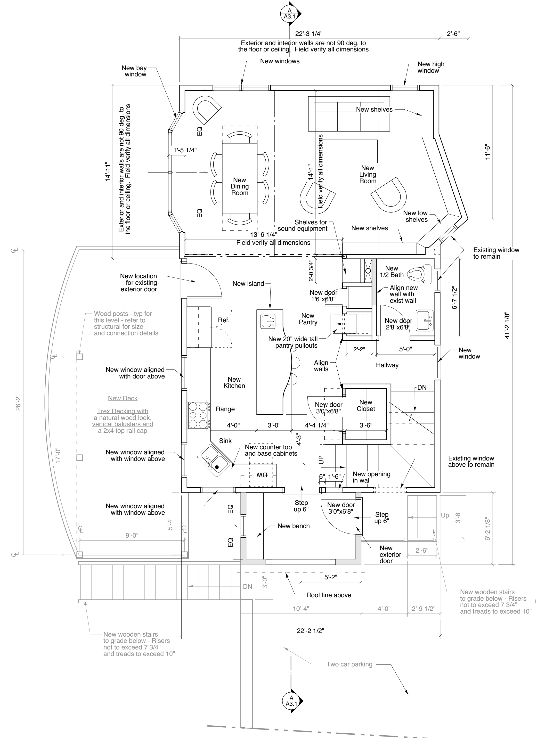
2 Main Level Floor Plan SCALE: 1/4" = 1'-0"
