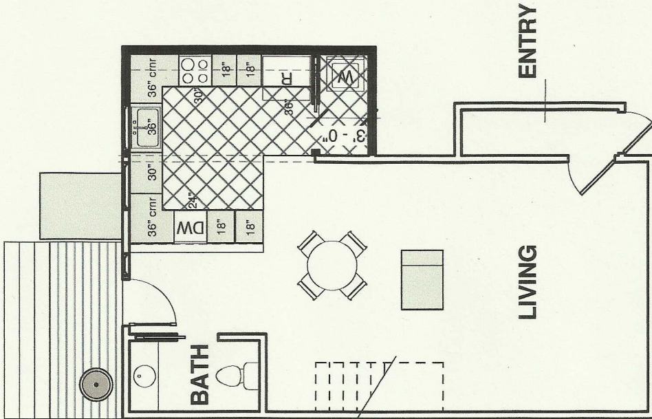
1 FIRST FLOOR PLAN 1/8" = 1'-0"
