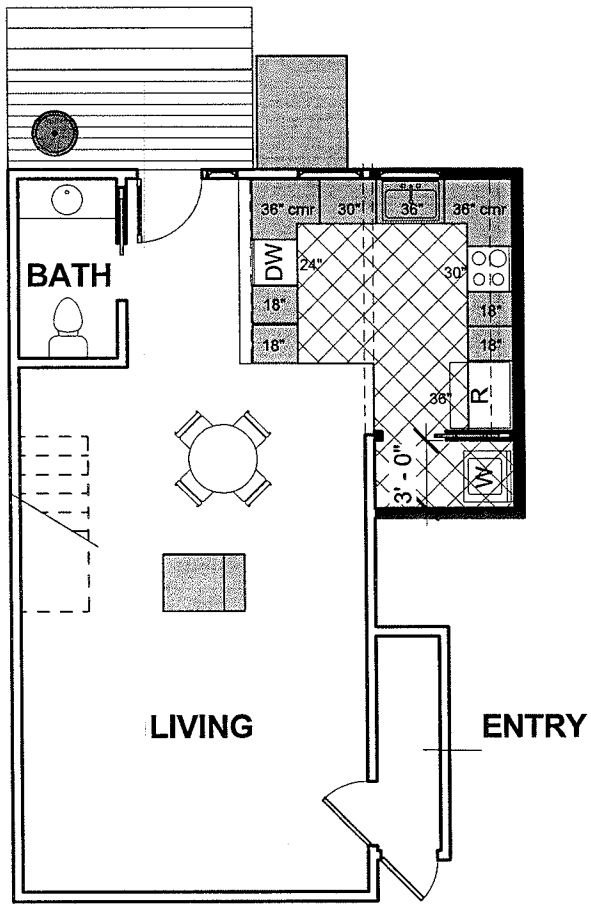
① FIRST FLOOR PLAN 1/8" = 1'-0"
