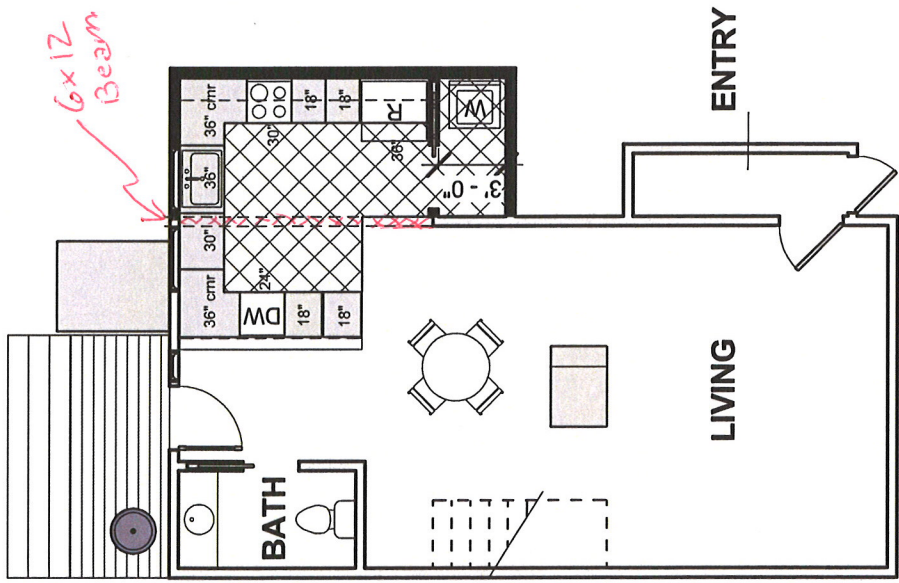
1 FIRST FLOOR PLAN 1/8" = 1'-0"
