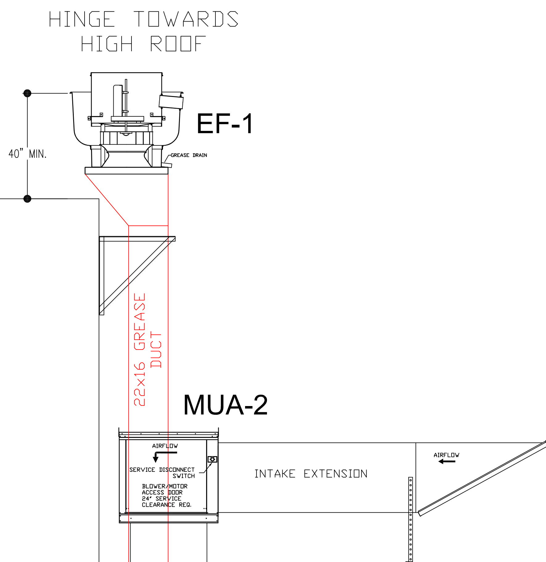
ROOF SIDE ELEVATION
