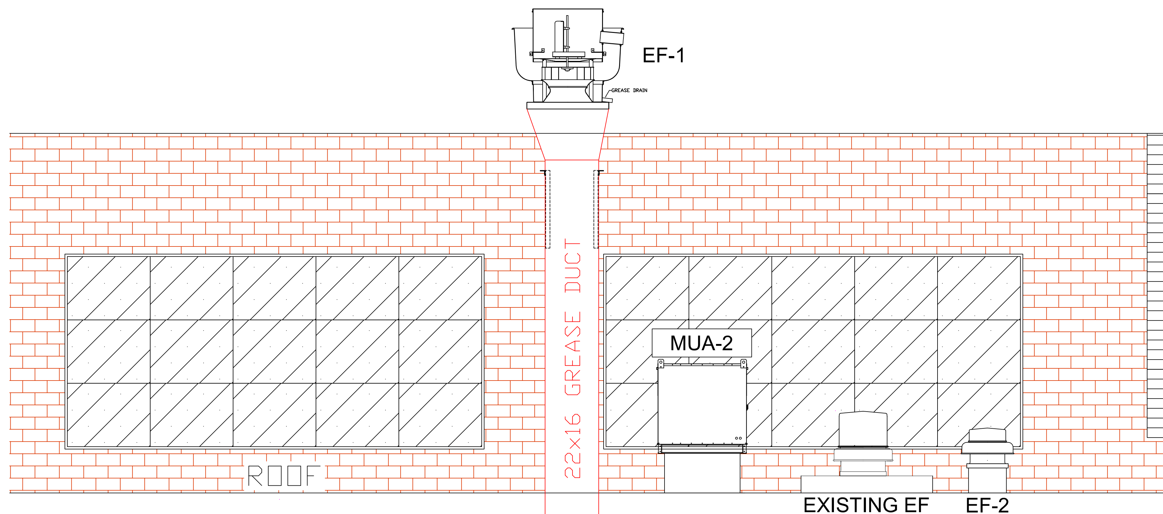
ROOF FRONT ELEVATION
