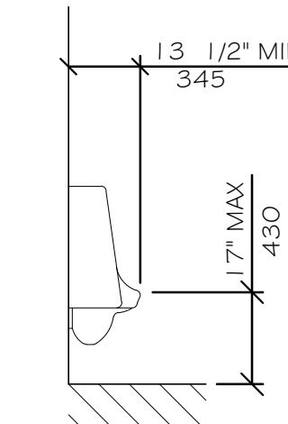
HEIGHT AND DEPTH OF URINAL NTS
