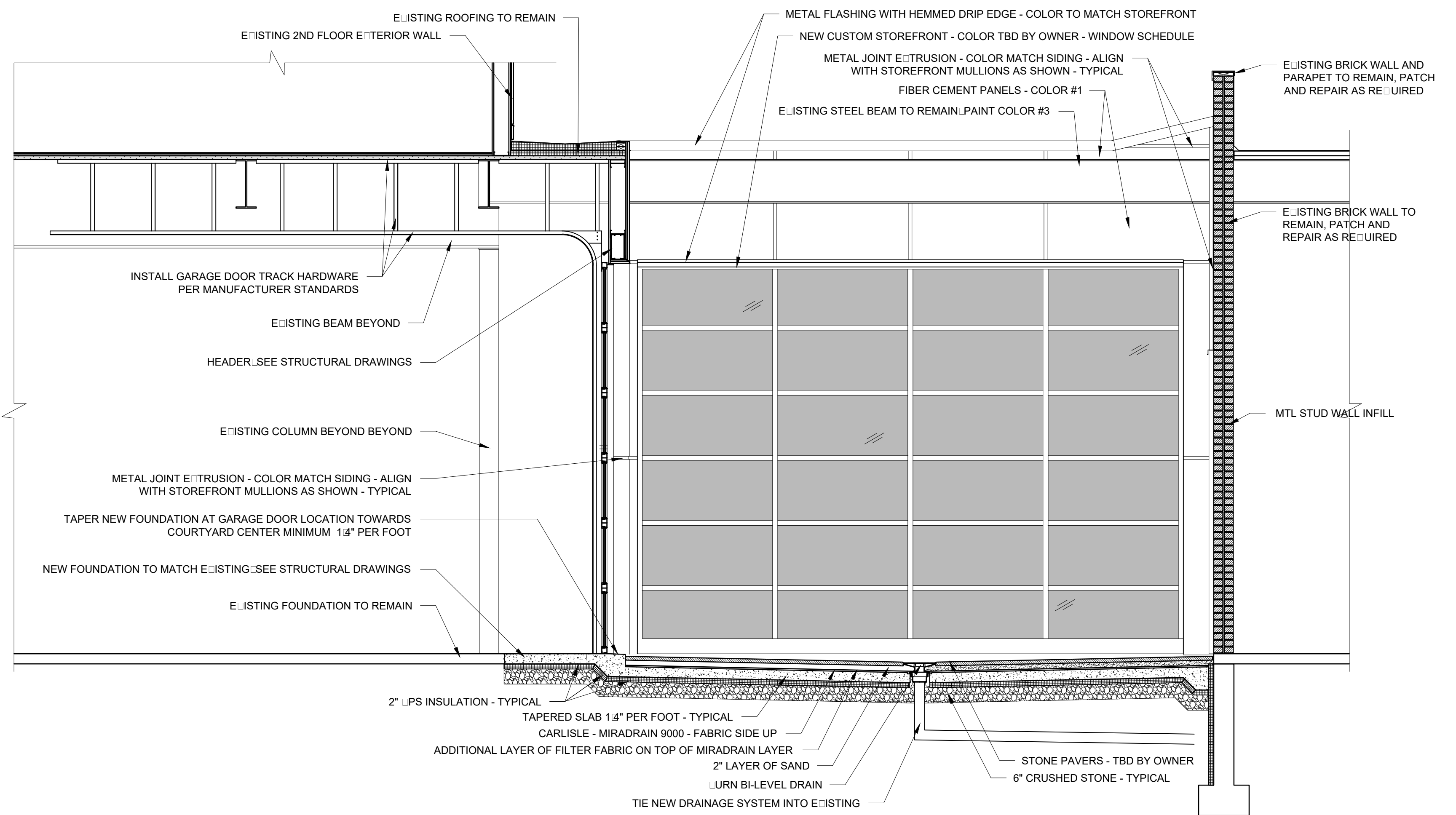
2 SECTION VIEW 1/2" = 1'-0"
