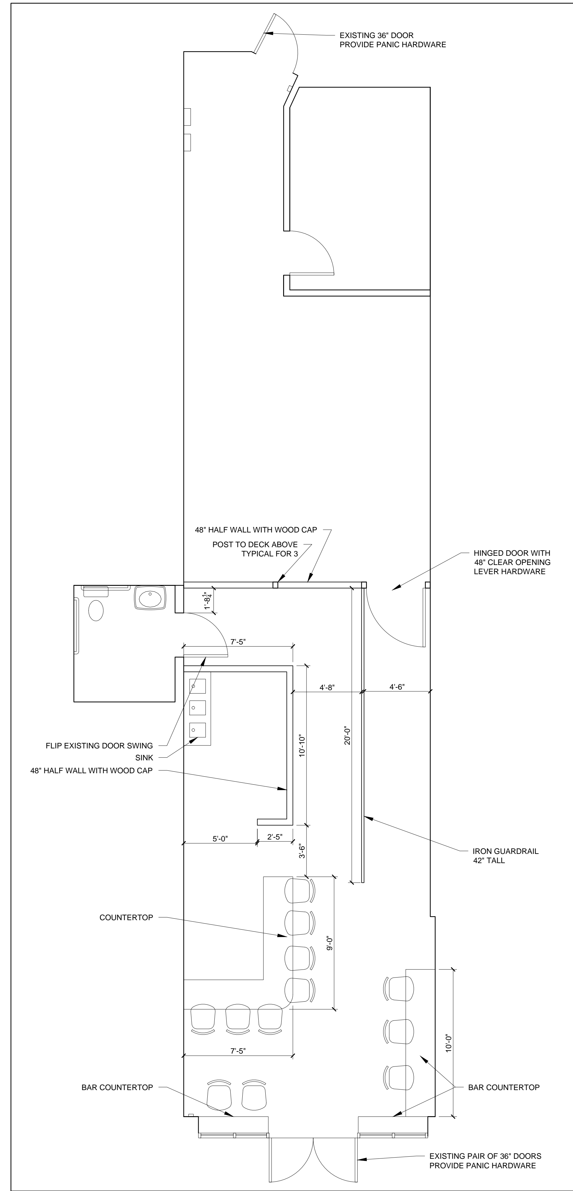
1 FLOOR PLAN 1/4" = 1'-0"
