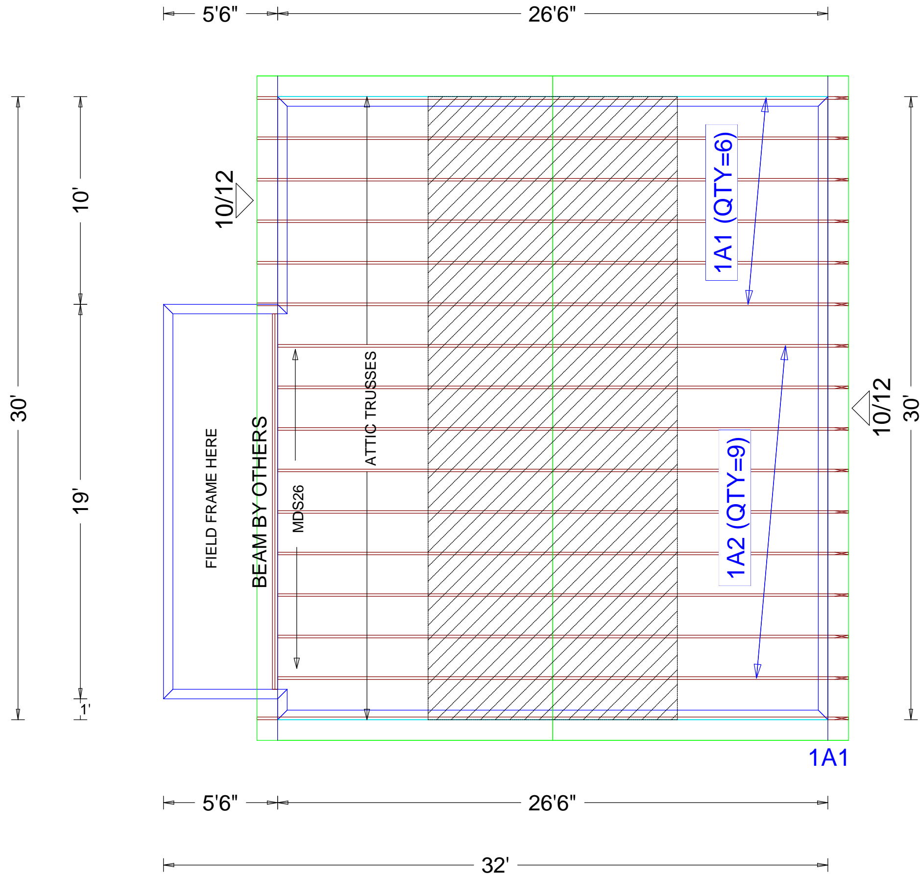
ROOF TRUSS LAYOUT -Not For Construction- BID SET-DRAFT 1
