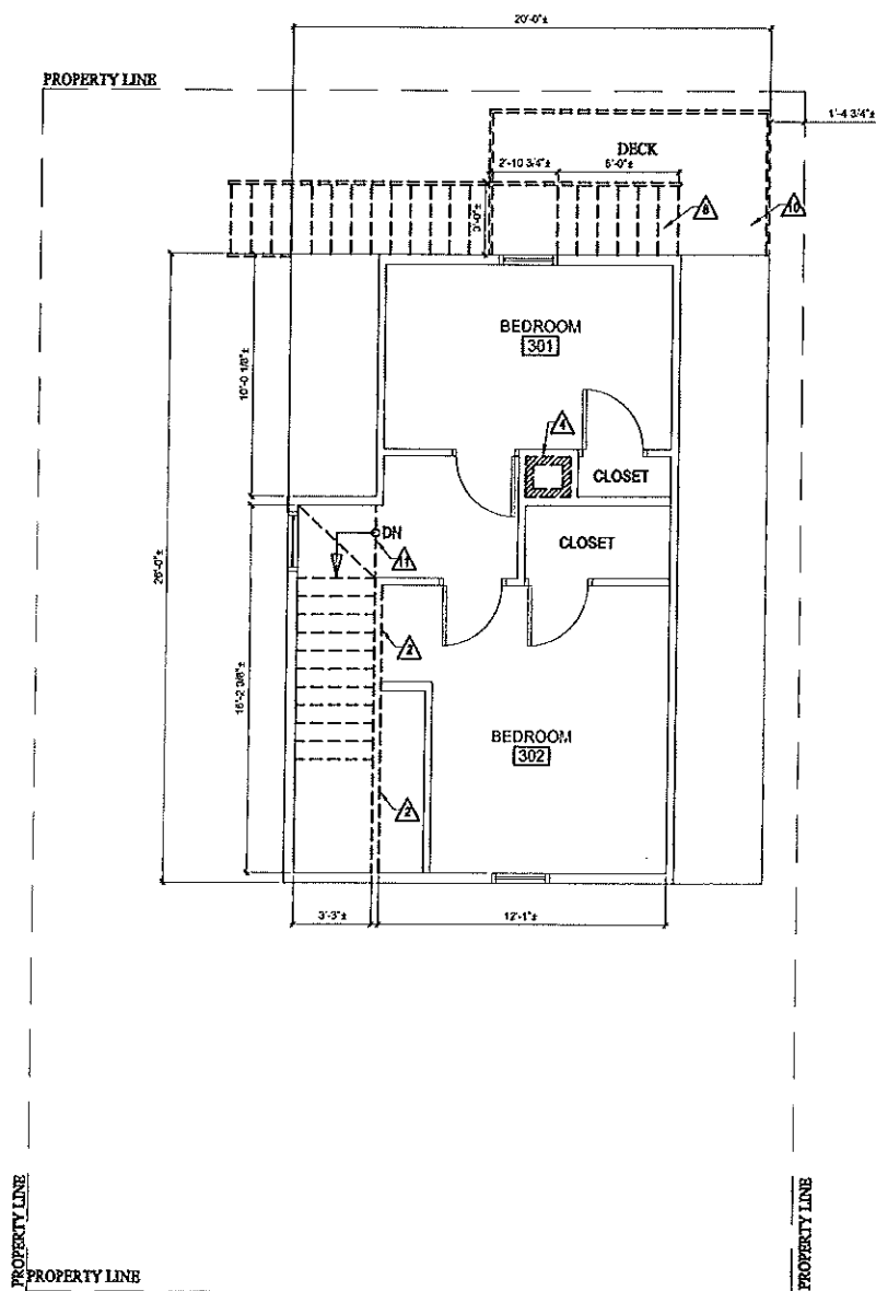
1 DEMO SECOND FLOOR AD102 SCALE: 1/4"=1'-0"
