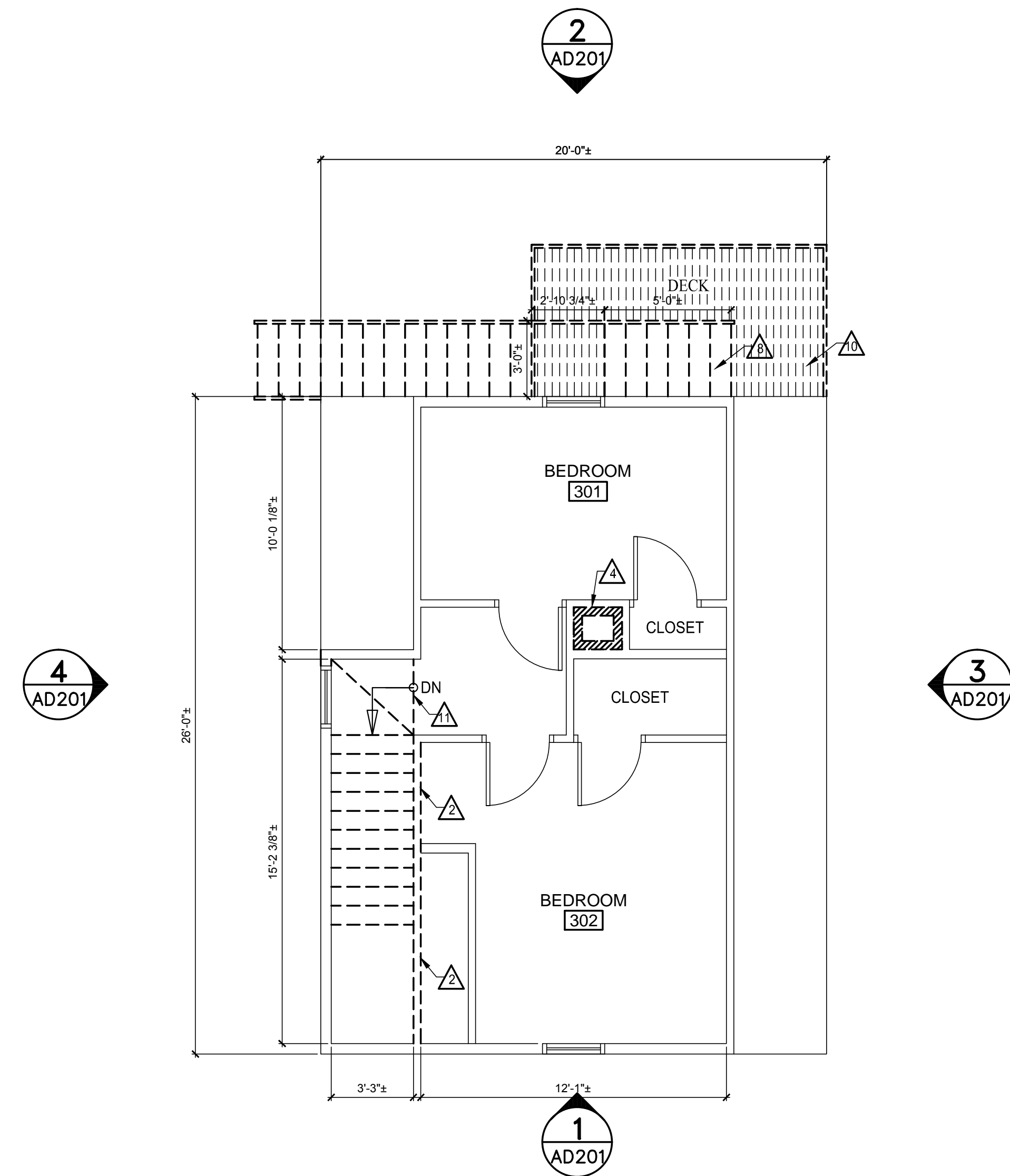
1 DEMO SECOND FLOOR AD102 SCALE: 1/4"=1'-0"
