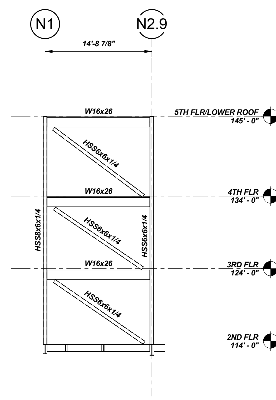
BF-6 AT LINE E4.2 1/8" = 1'-0"
