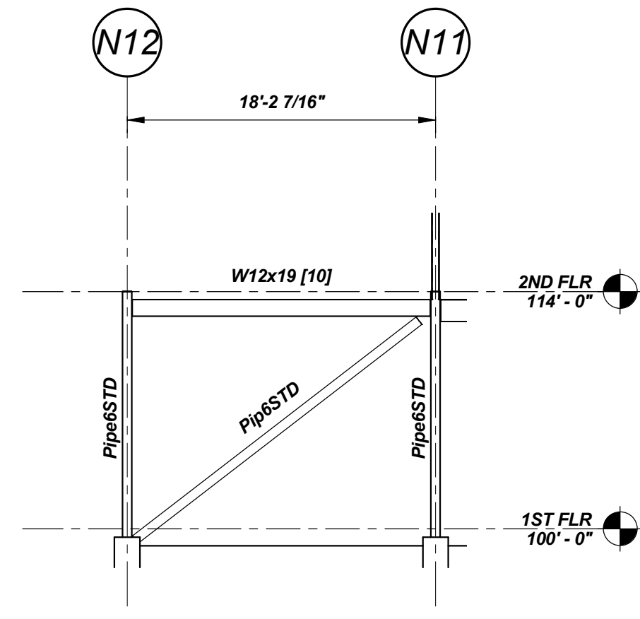
BF-1 AT LINE W8 1/8" = 1'-0"
