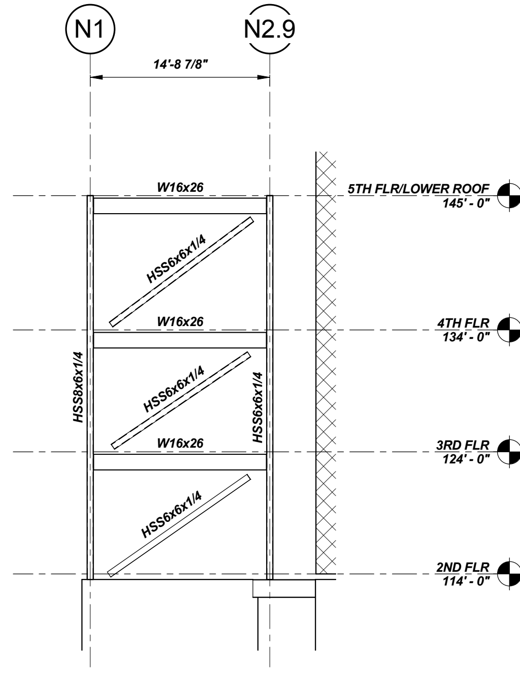
BF-5 AT LINE E8.3 1/8" = 1'-0"
