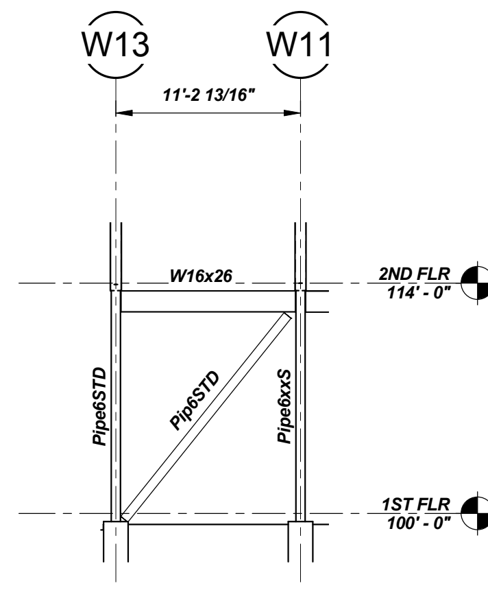
BF-3 AT LINE N11 1/8" = 1'-0"
