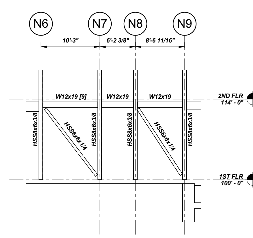
BF-4 AT LINE W14 1/8" = 1'-0"
