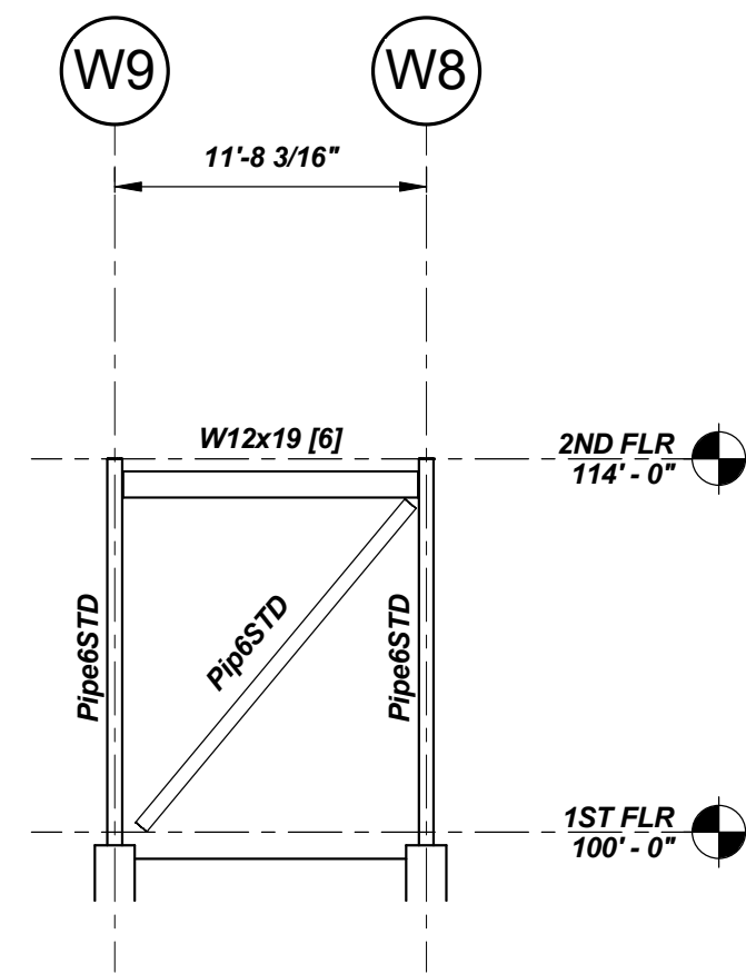
BF-2 AT LINE N12 1/8" = 1'-0"
