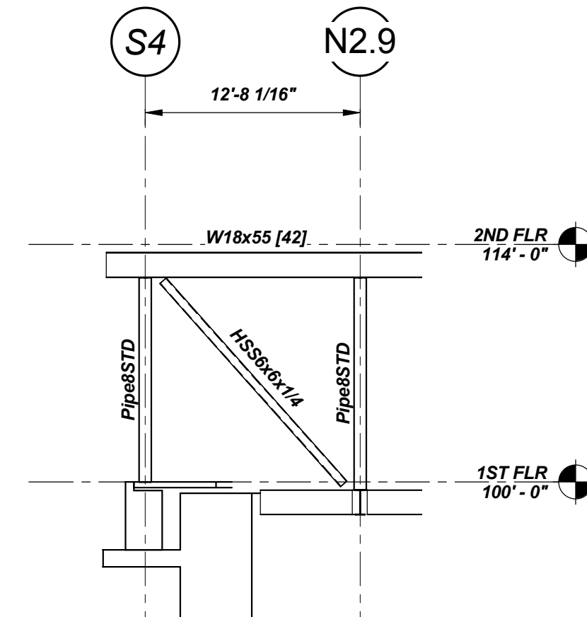
BF-7 AT LINE E2.4 1/8" = 1'-0"
