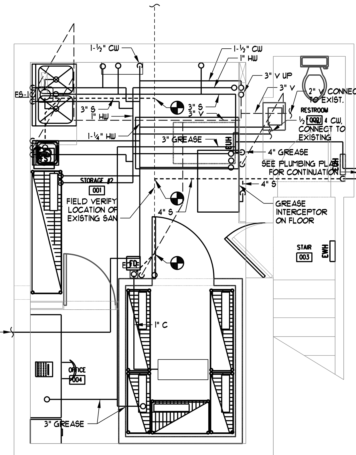
BASEMENT PLUMBING PLAN SCALE - 3/8" = 1'-0"
