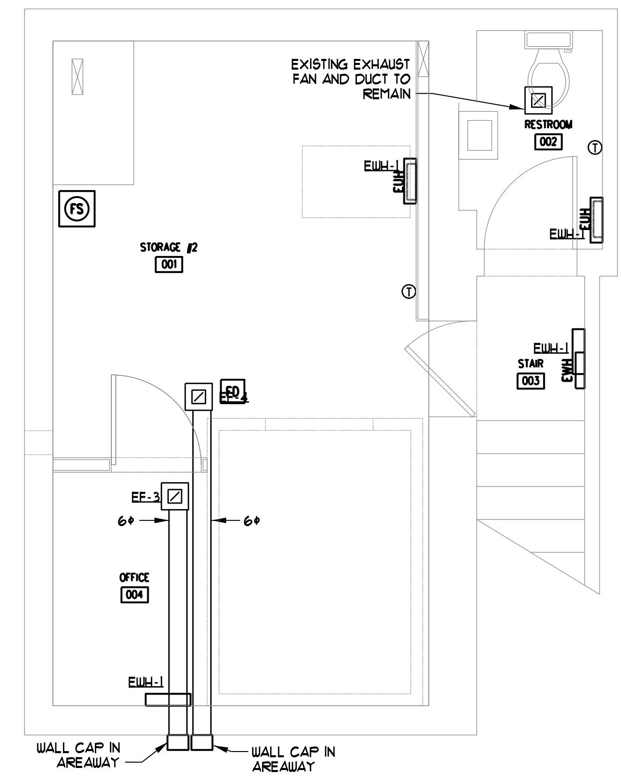
BASEMENT MECHANICAL PLAN SCALE - 3/8" = 1'-0"
