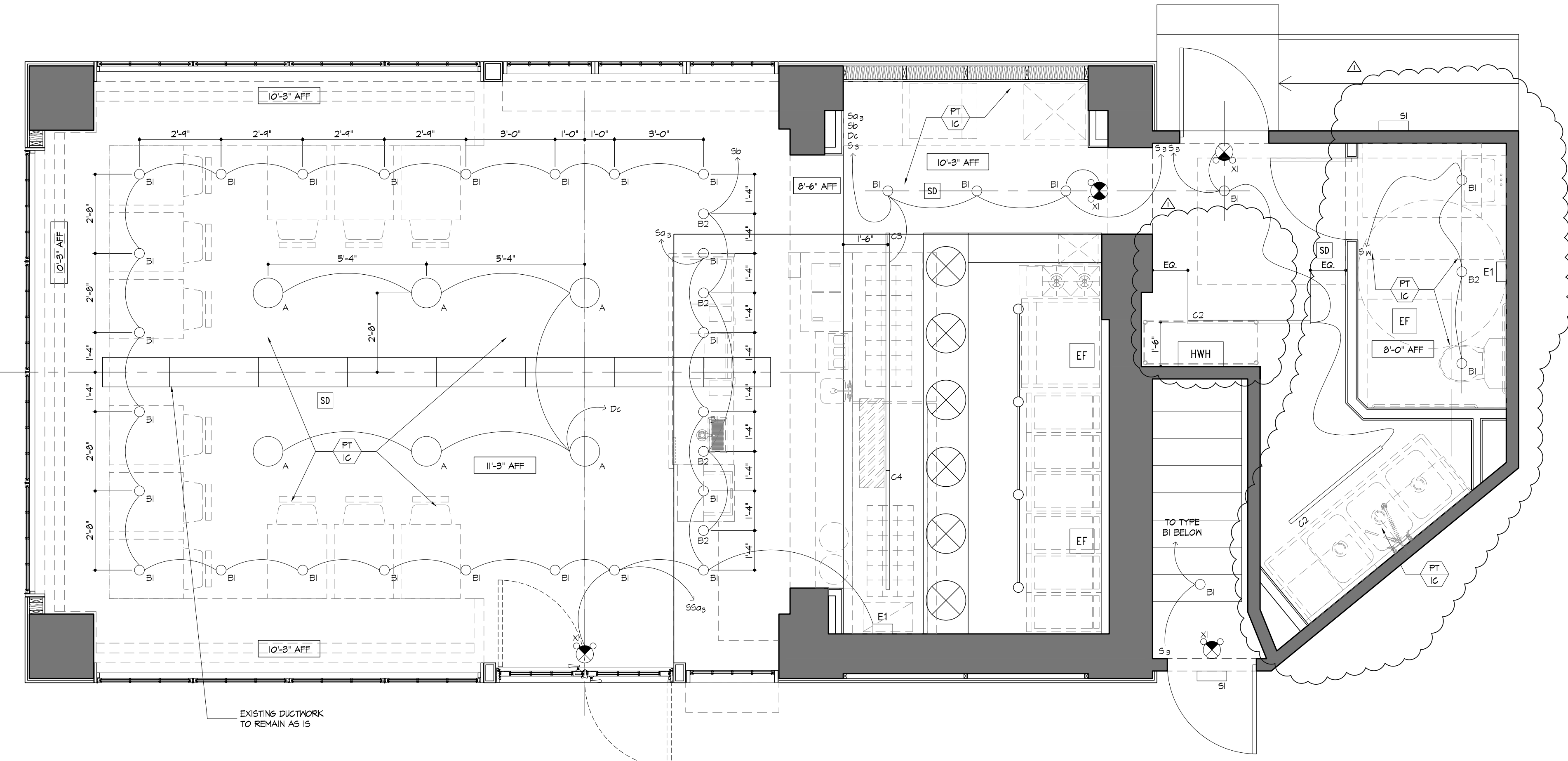
1 Reflected Ceiling Plan: Ground Floor Scale: 3/8" = 1'-0"
