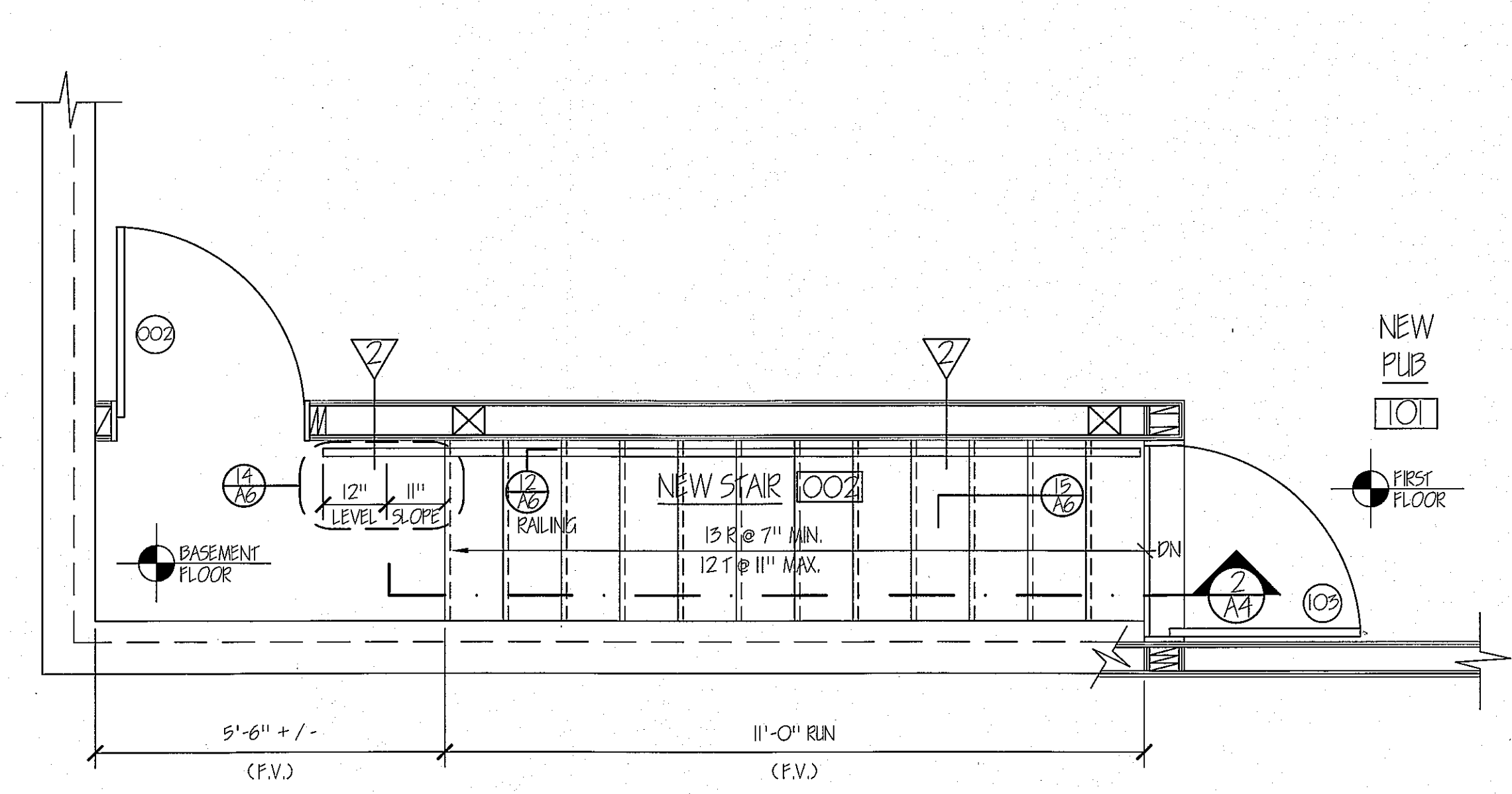
(1) PLAN AT NEW STAIR SCALE: 1/2" = 1'-0"
