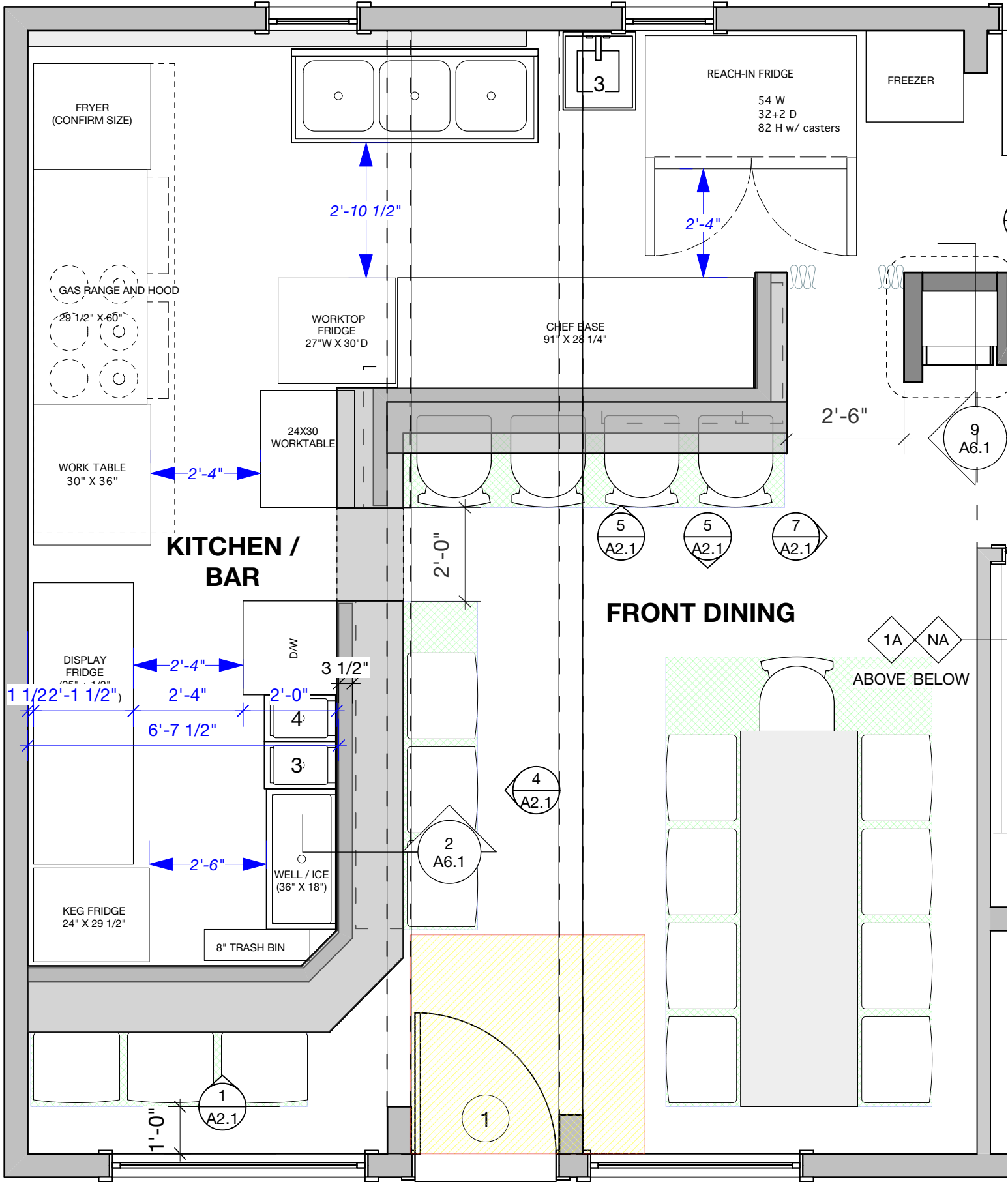
1 KITCHEN PLAN Scale: 3/8" = 1'-0"
