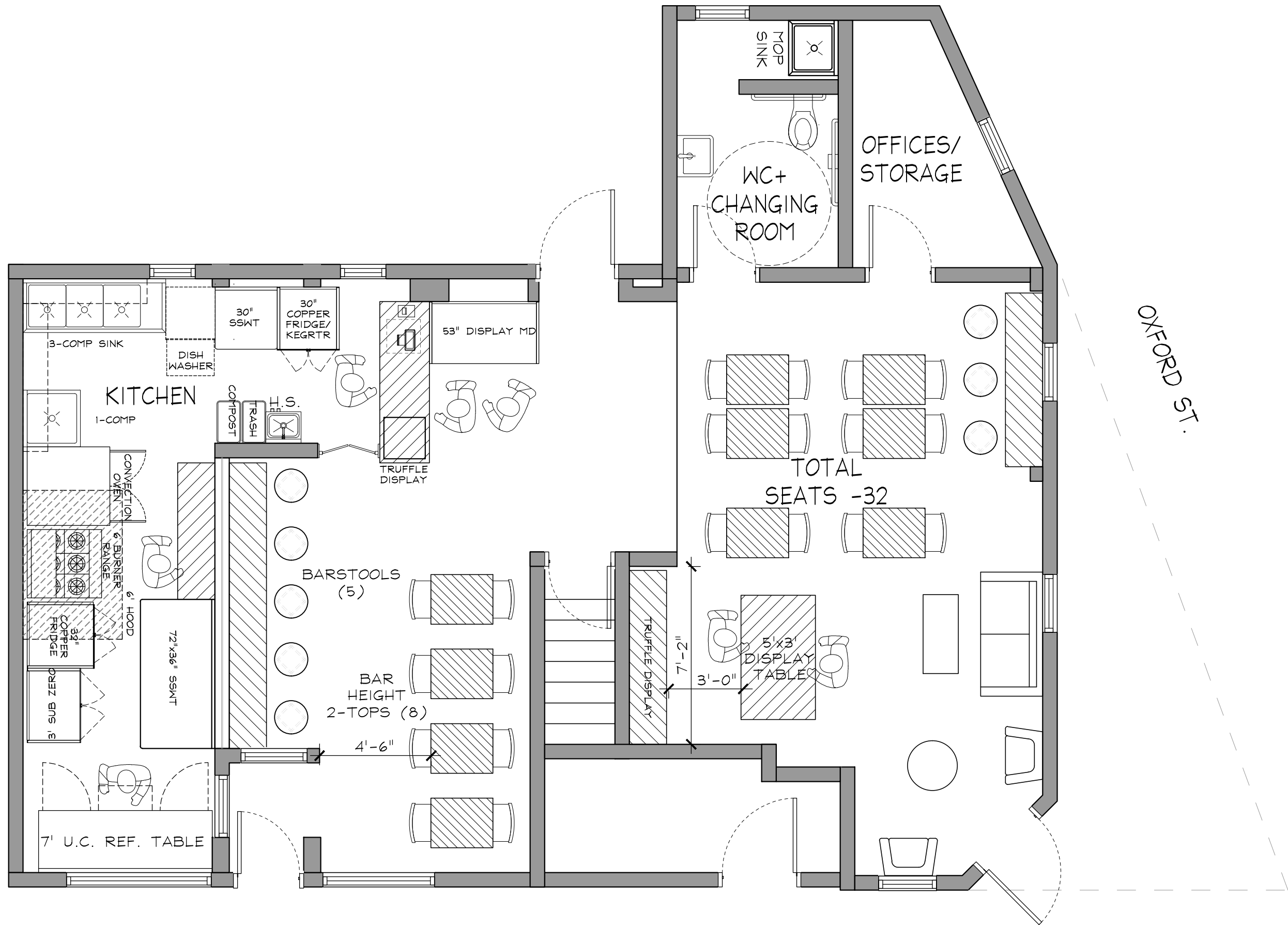
1 Fixture Plan Scale: 1/4" = 1' - 0"
