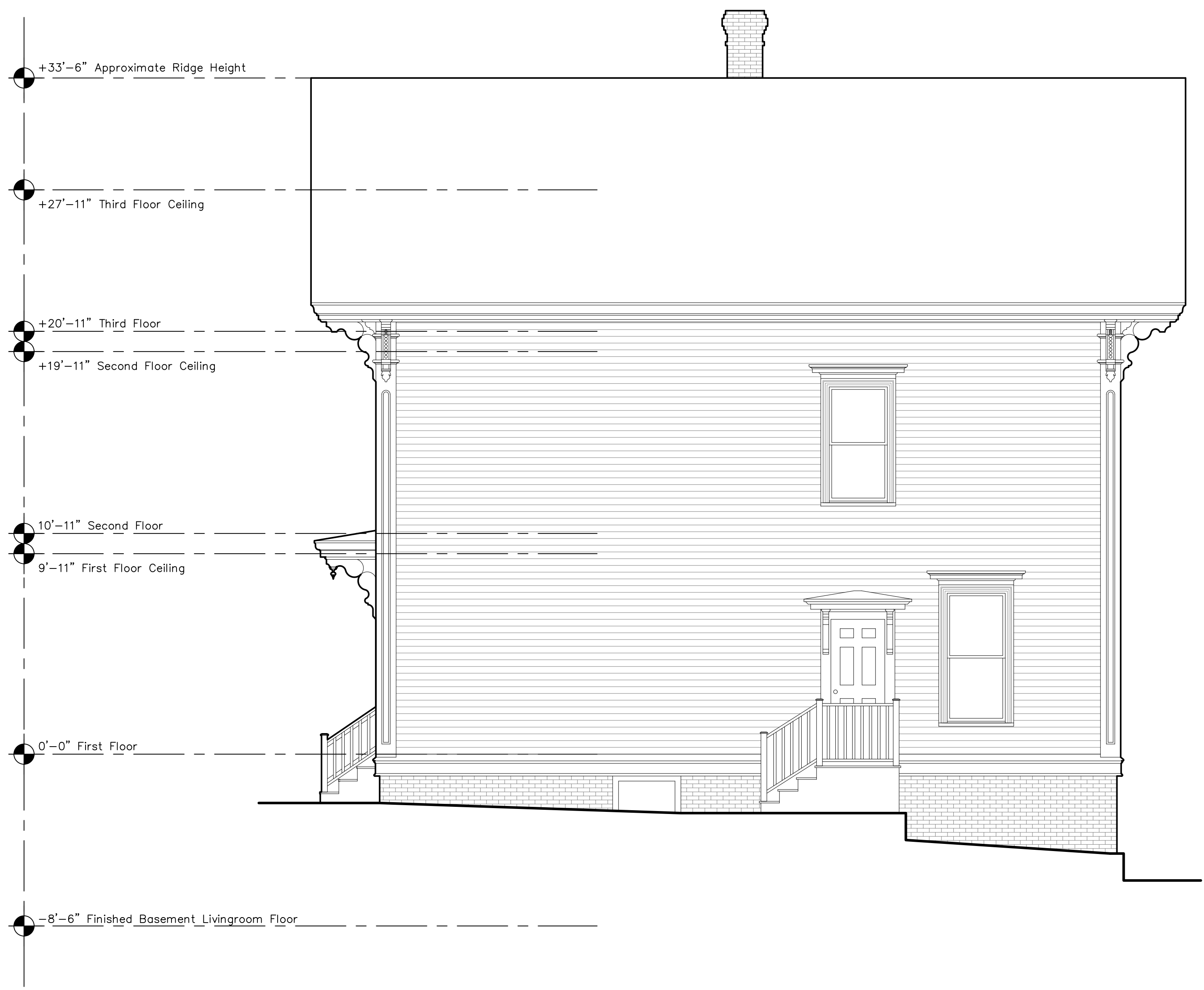
1 EXISTING EAST ELEVATION 1/4"=1'-0"
