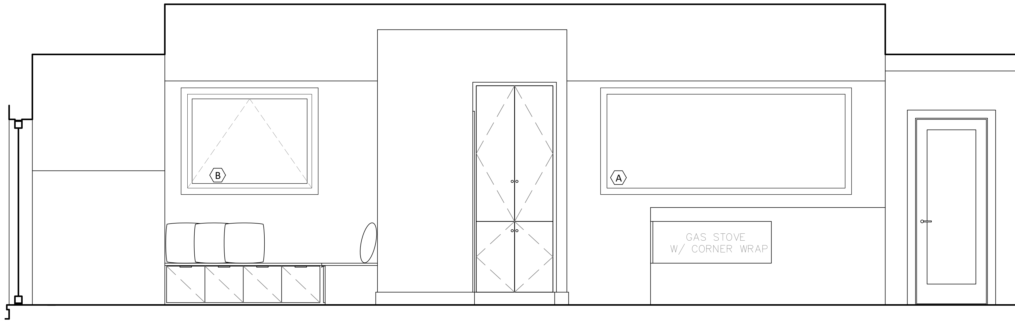
1 ELEVATION EAST 1/2" = 1'-0"
