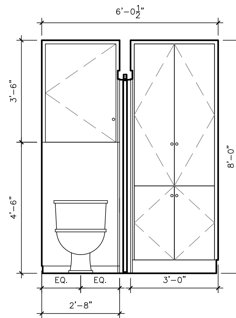
2 ELEVATION EAST 1/2"=1'-0"
