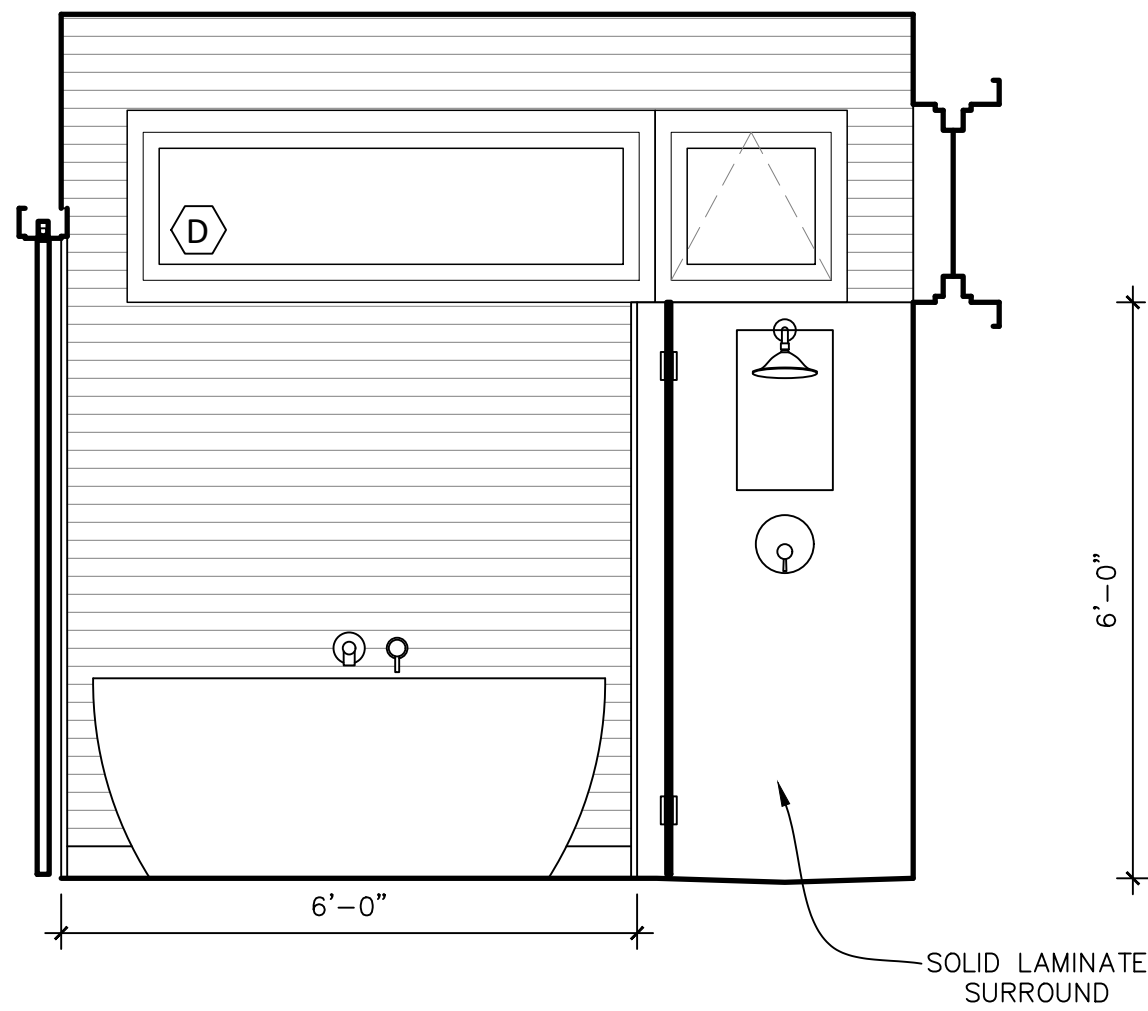
4 ELEVATION NORTH @ SHOWER 1/2"=1'-0"
