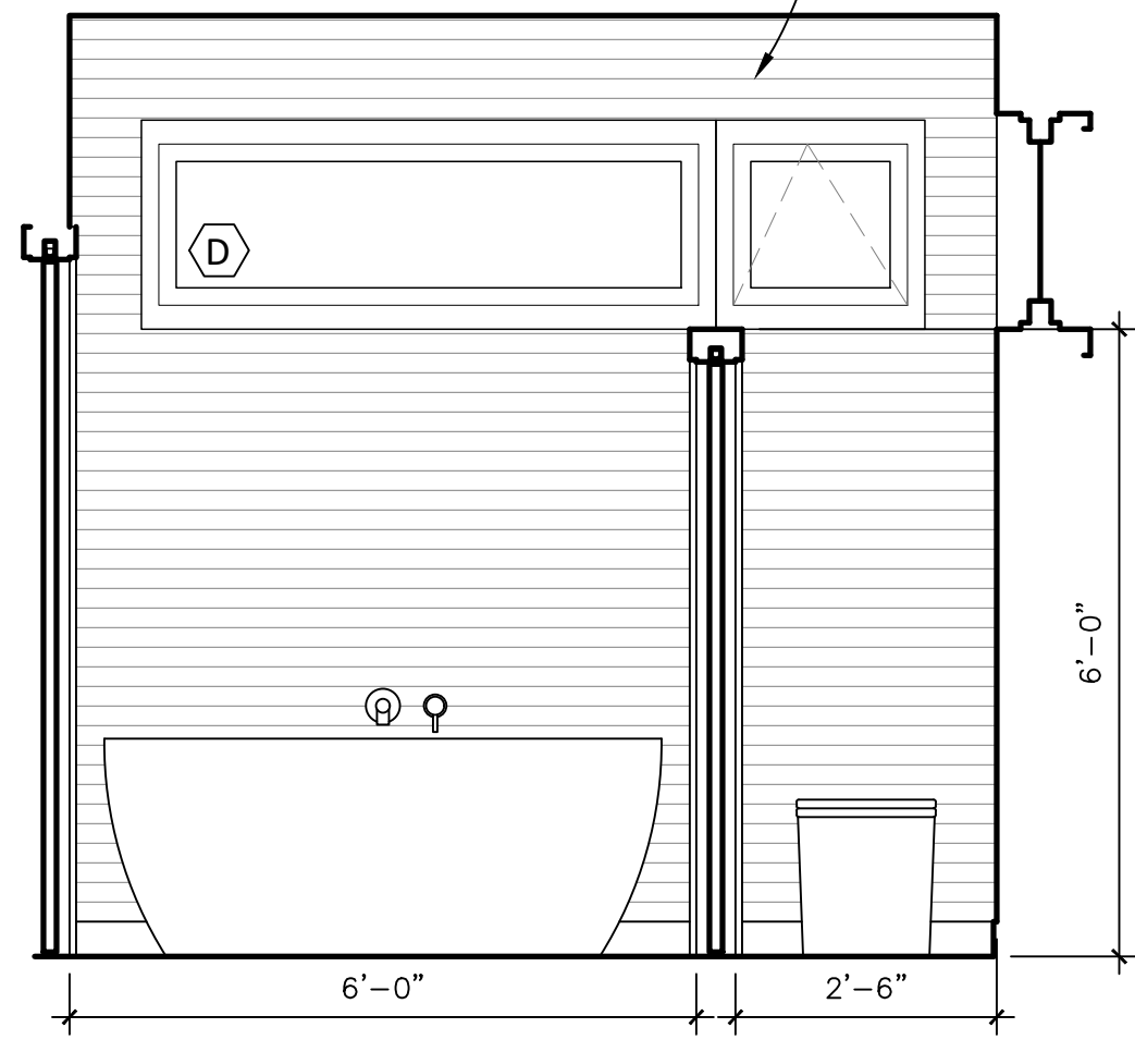
6 ELEVATION NORTH @ WATER CLOSET 1/2"=1'-0"
