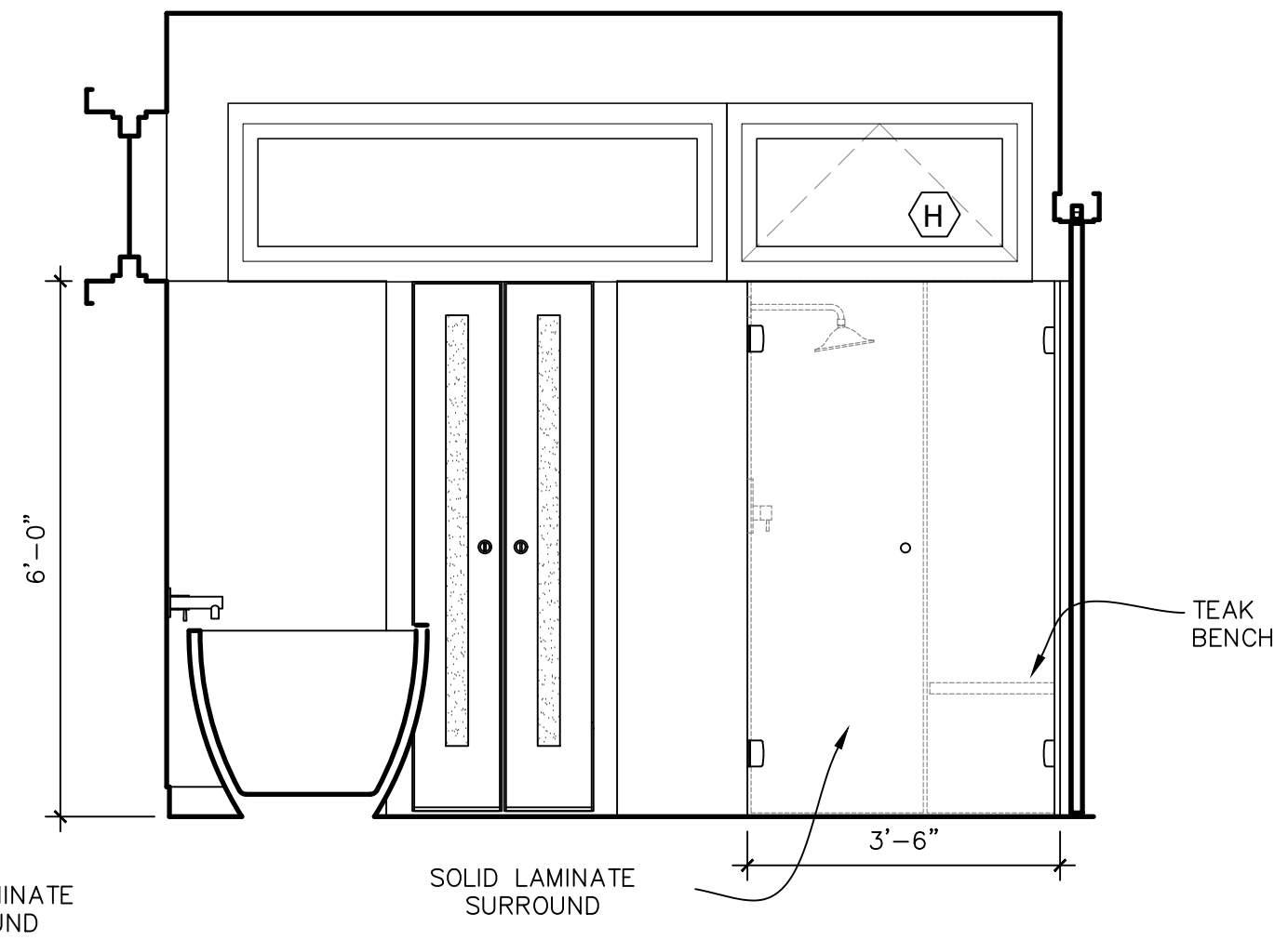
2 ELEVATION EAST 1/2"=1'-0"
