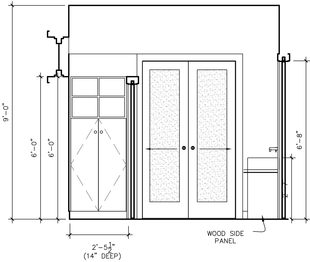
5 ELEVATION SOUTH @ WATER CLOSET 1/2"=1'-0"
