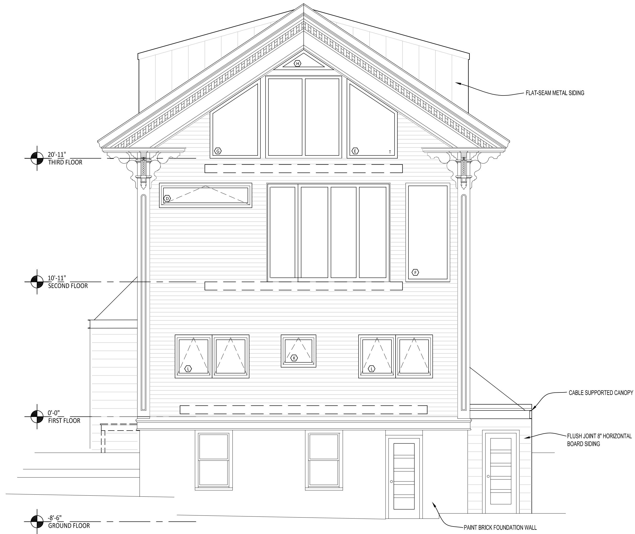
1 NORTH ELEVATION 1/4" = 1'-0"
