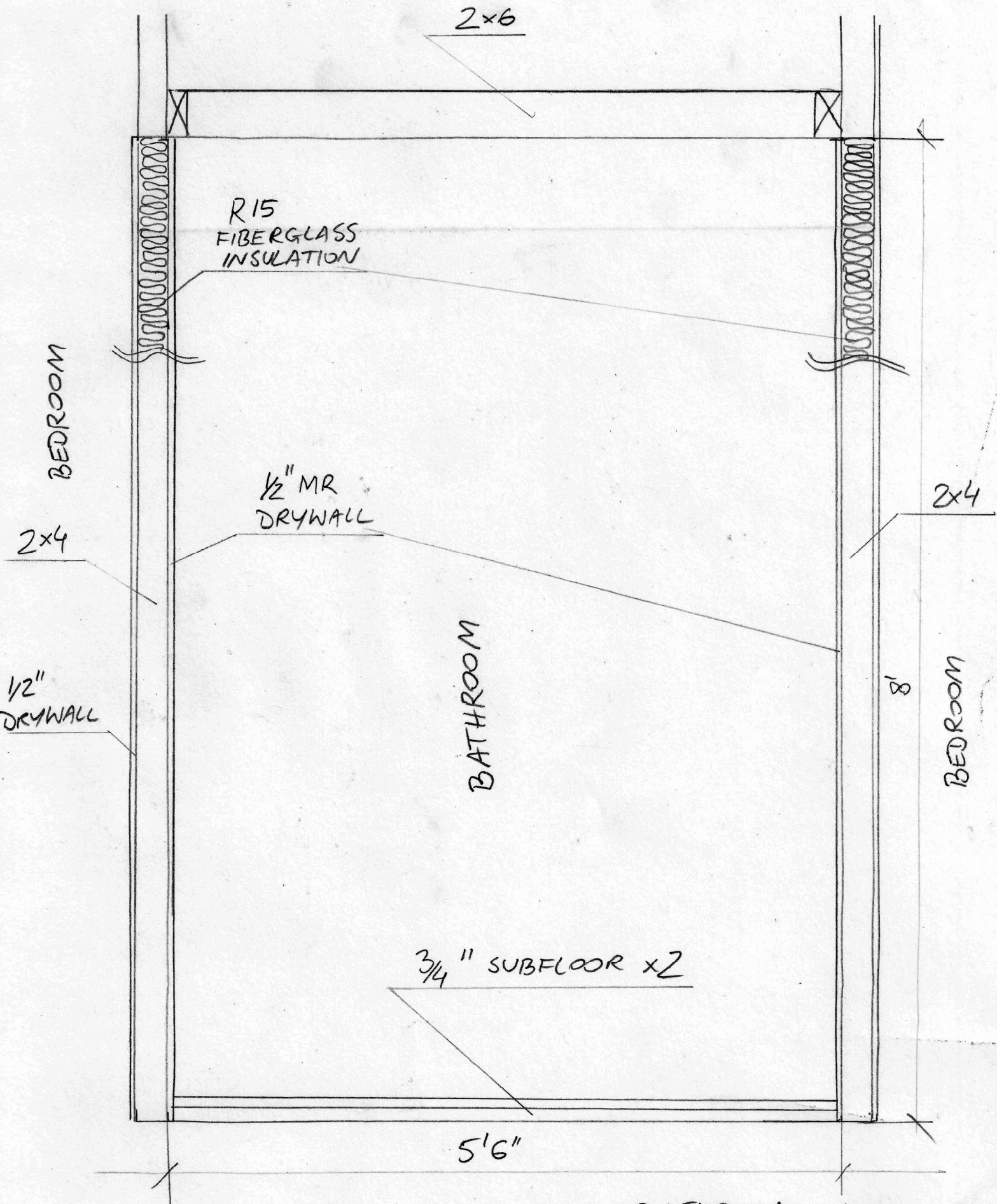
BATHROOM WALL CROSS SECTION
