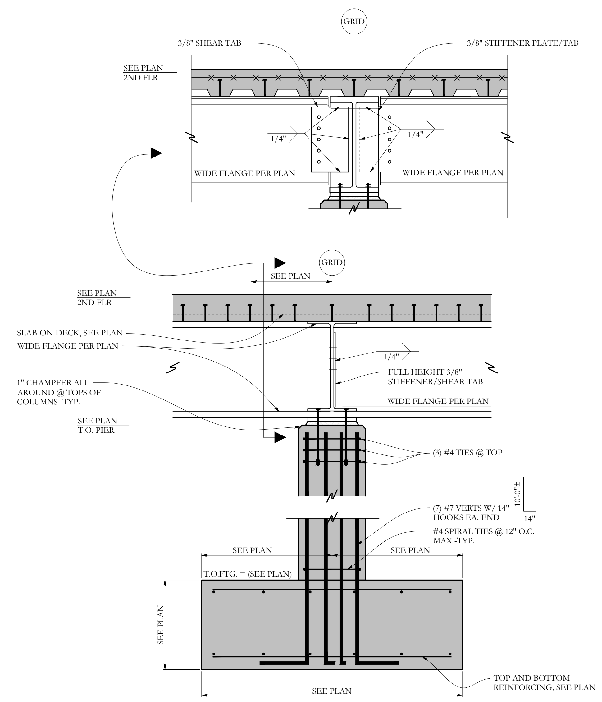
SECTION A S-3.3 3/4"=1'-0"
