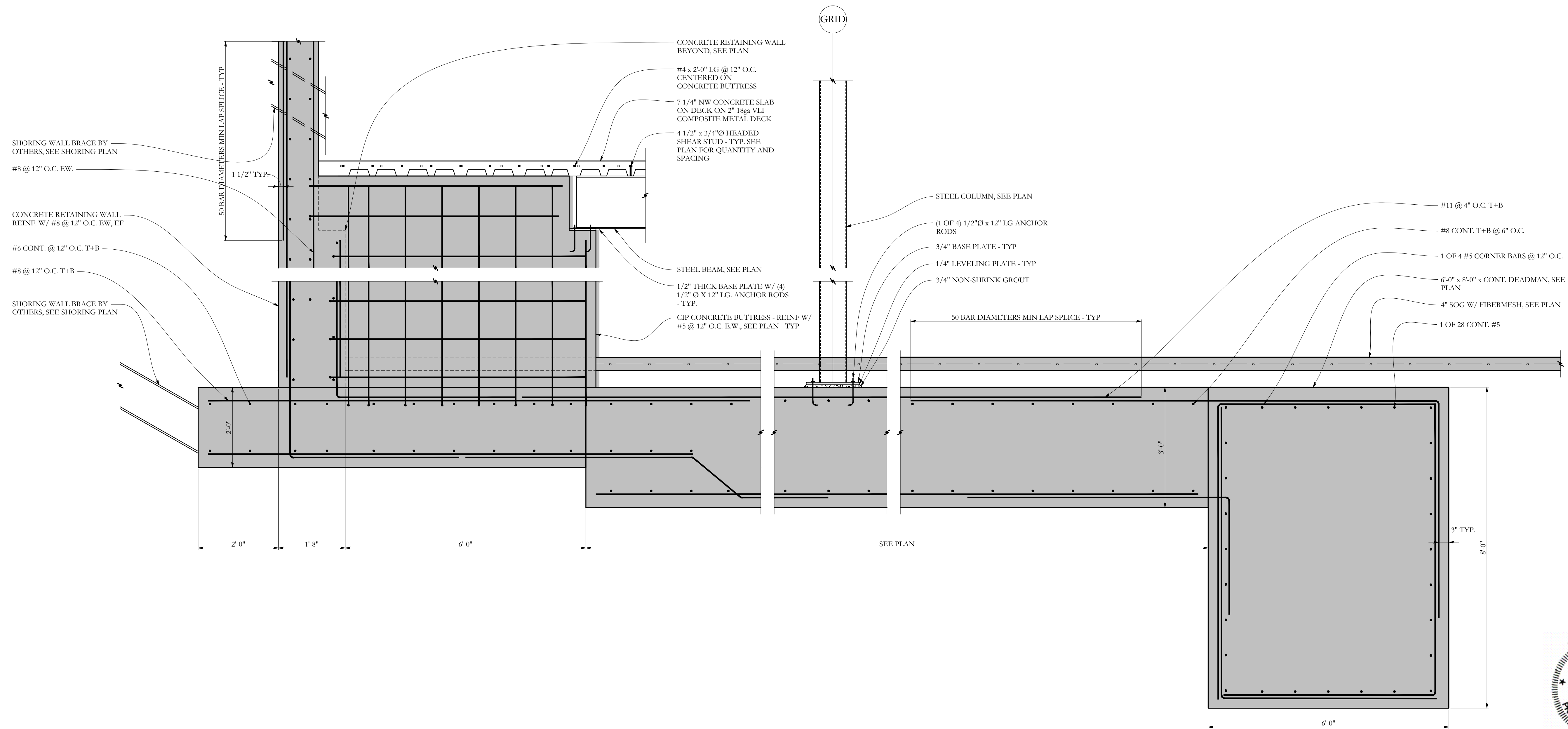
SECTION A 3/4"=1'-0
