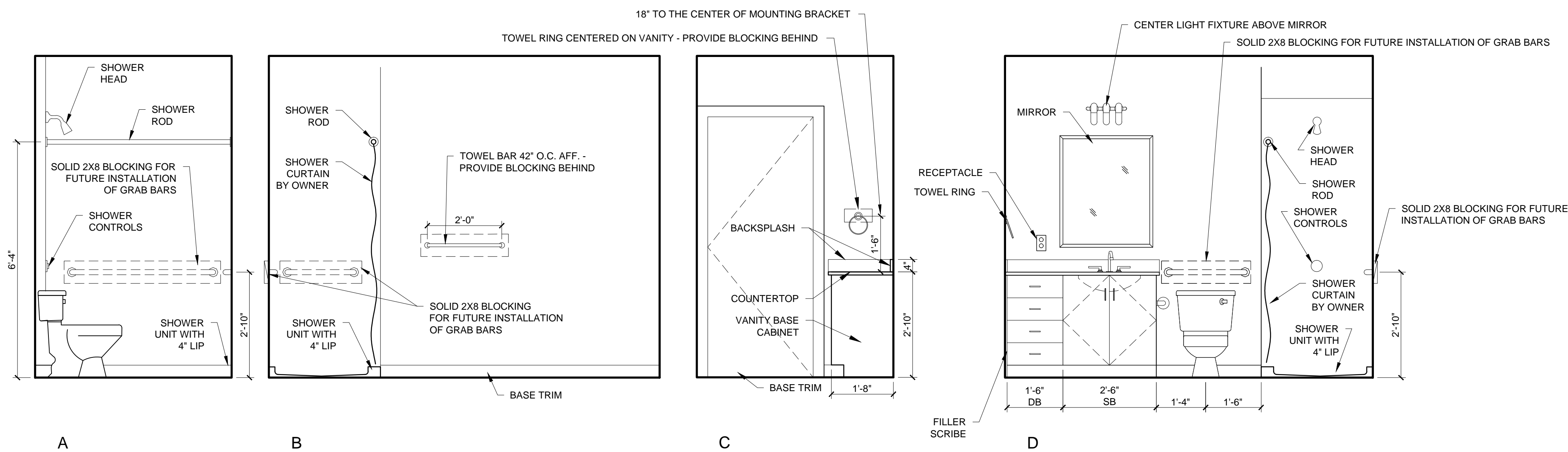
3 UNIT 404 - BATH WITH SHOWER - INTERIOR ELEVATIONS 1/2" = 1'-0"
