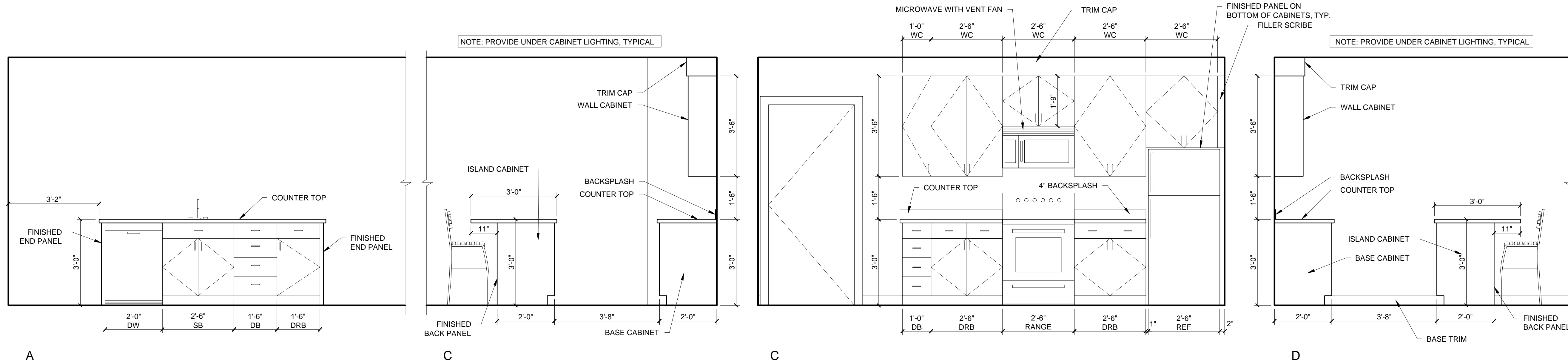
1 UNIT 404 - KITCHEN - INTERIOR ELEVATIONS 1/2" = 1'-0"
