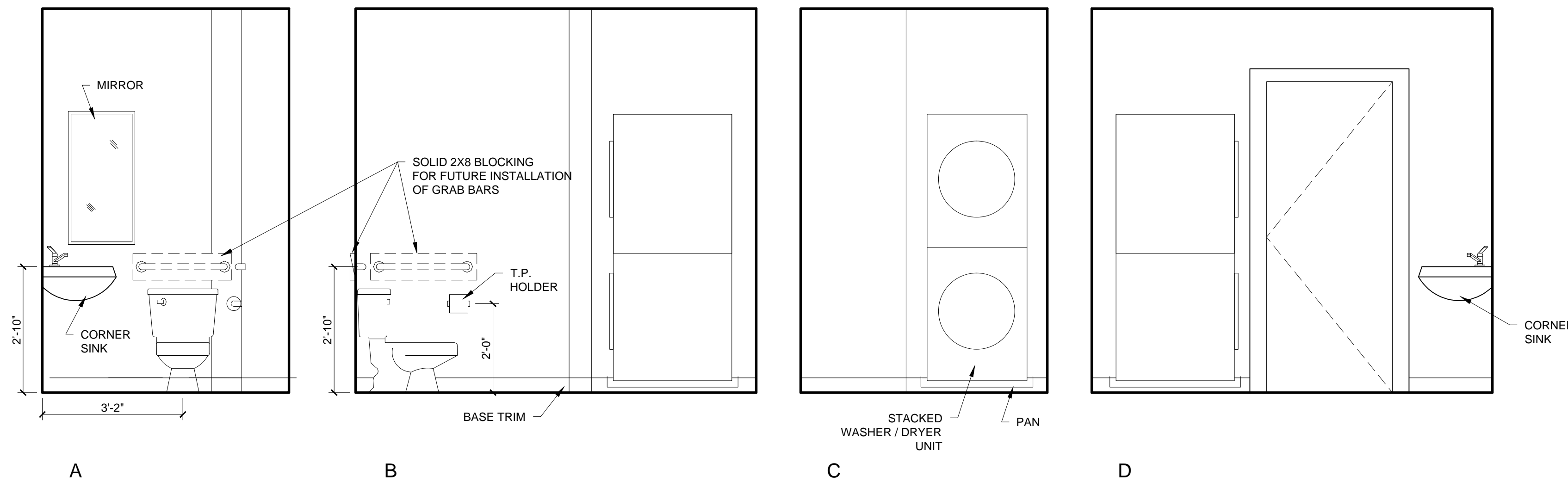
2 UNIT 404 - HALF BATH - INTERIOR ELEVATIONS 1/2" = 1'-0"
