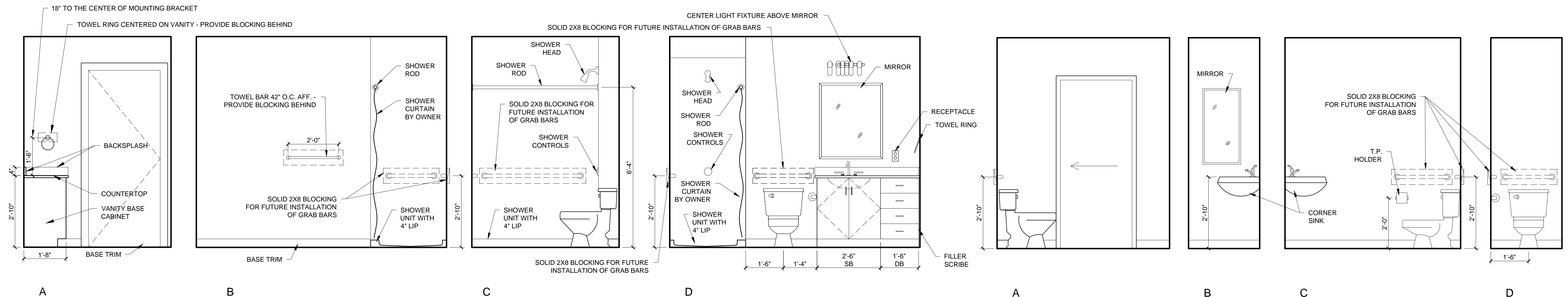
3 UNIT 304 - BATHROOM WITH SHOWER - INTERIOR ELEVATIONS 1/2" = 1'-0"
