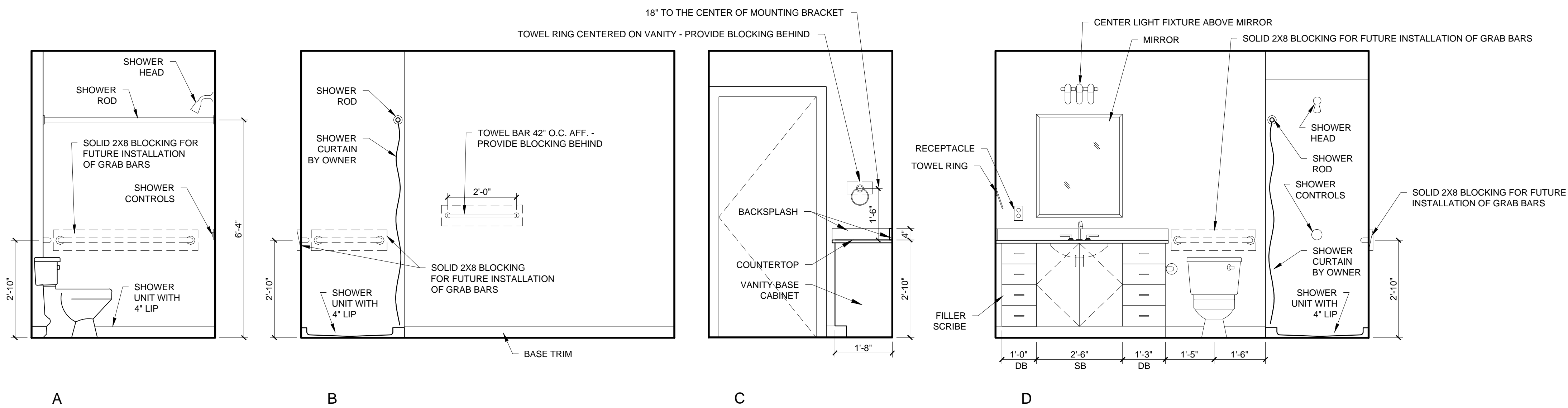
3 UNIT 303 - BATHROOM WITH SHOWER - INTERIOR ELEVATIONS 1/2" = 1'-0"
