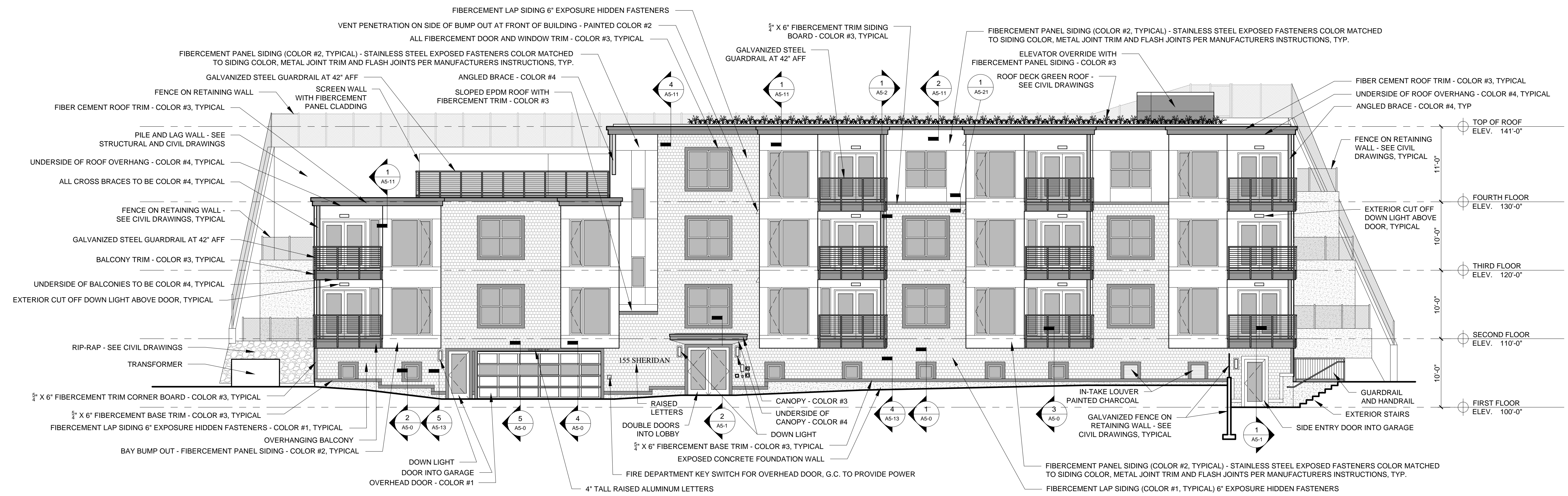
1 WEST ELEVATION 1/8" = 1'-0"
