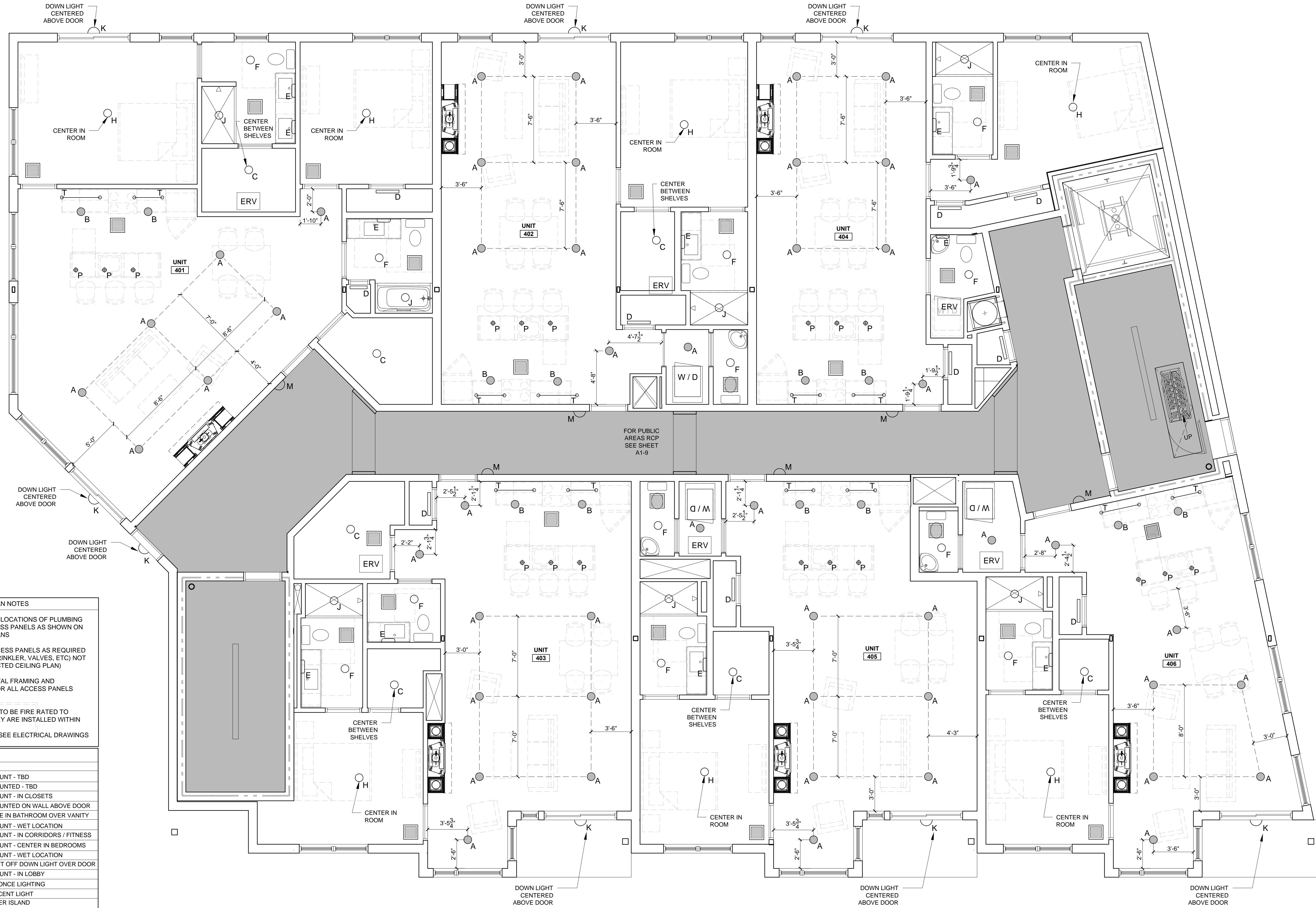
1 UNIT 401-406 REFLECTED CEILING PLAN 1/4" = 1'-0"
