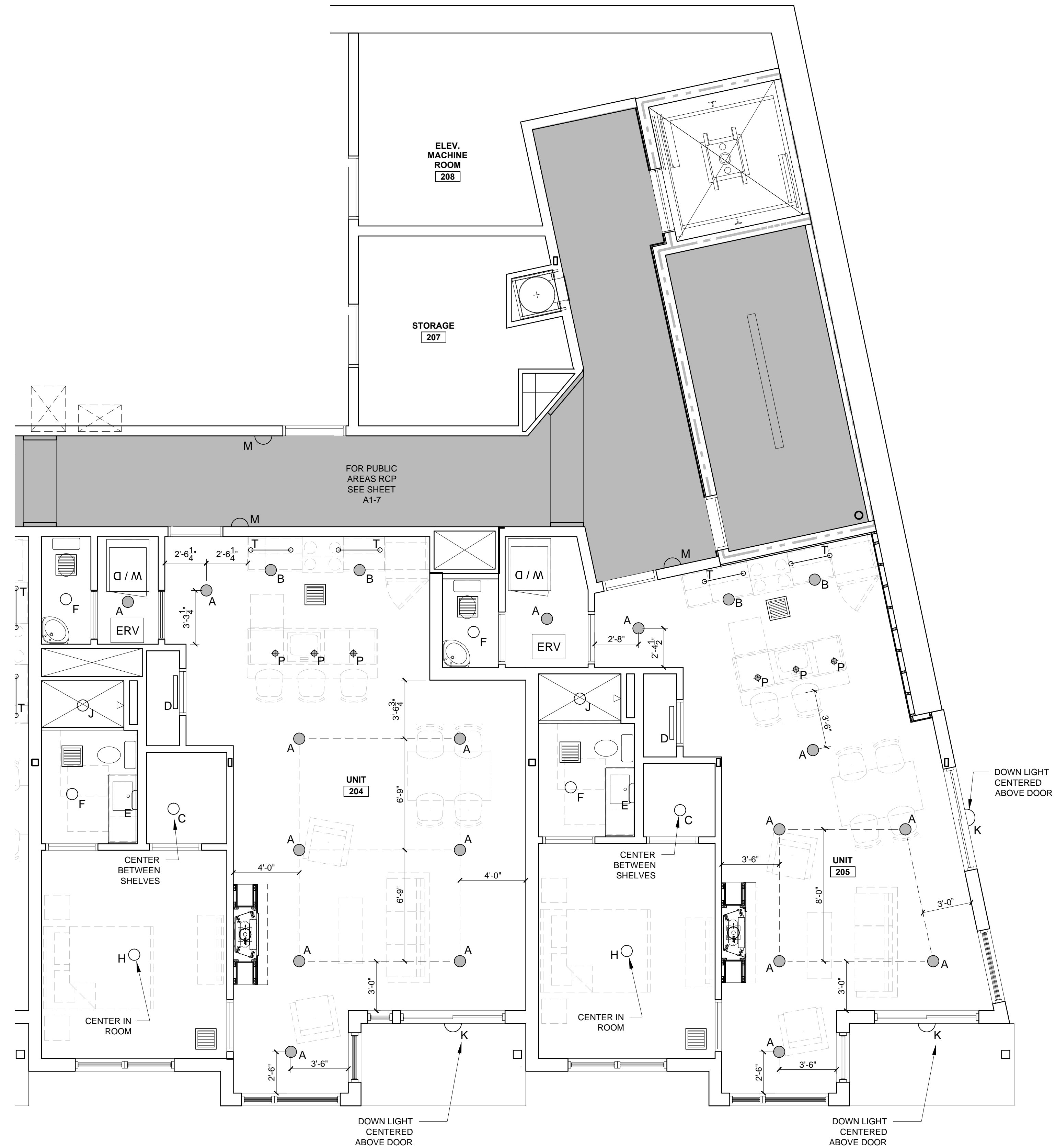
1 UNIT 204-205 REFLECTED CEILING PLAN 1/4" = 1'-0"
