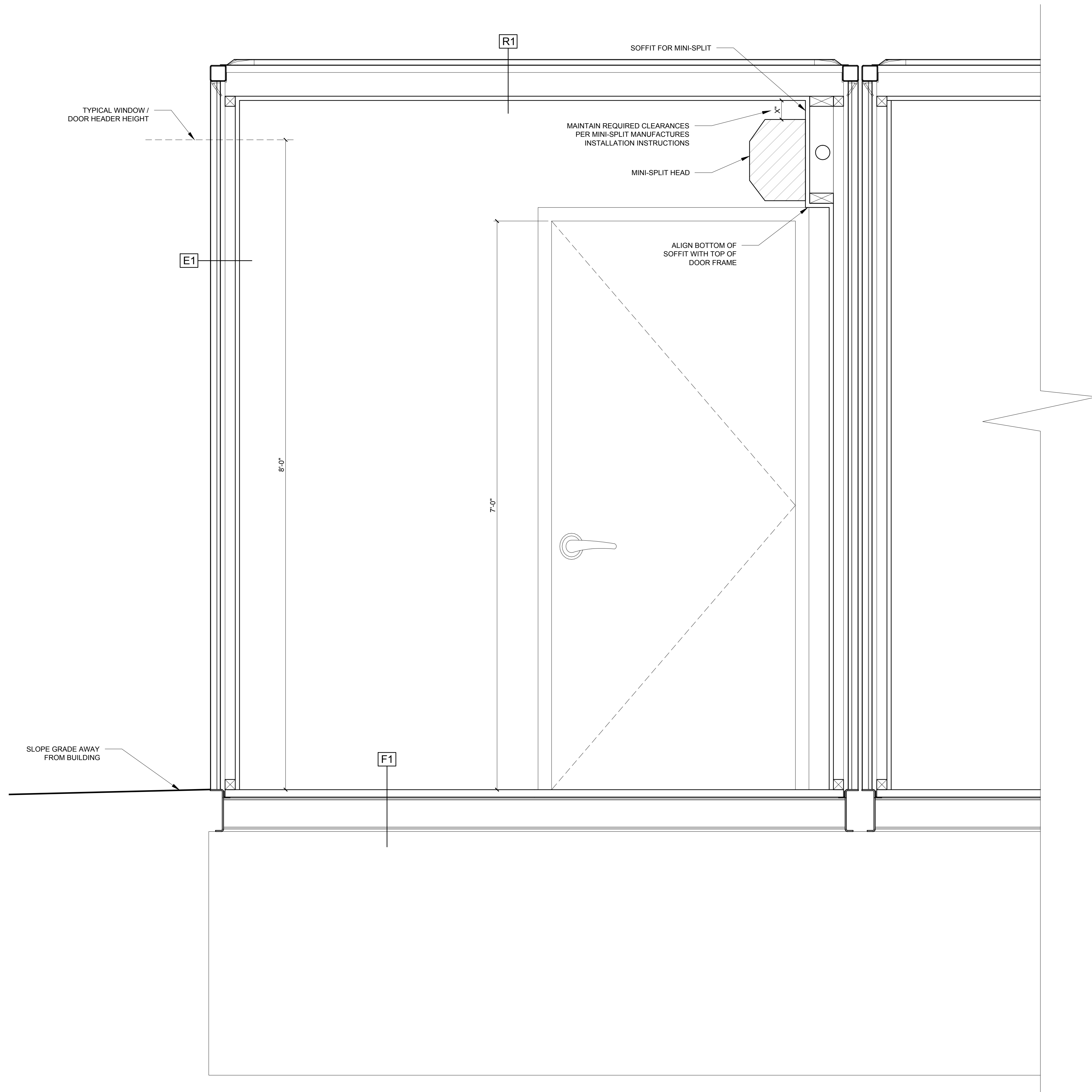
1 TYPICAL SECTION 1/12" = 1'-0"
