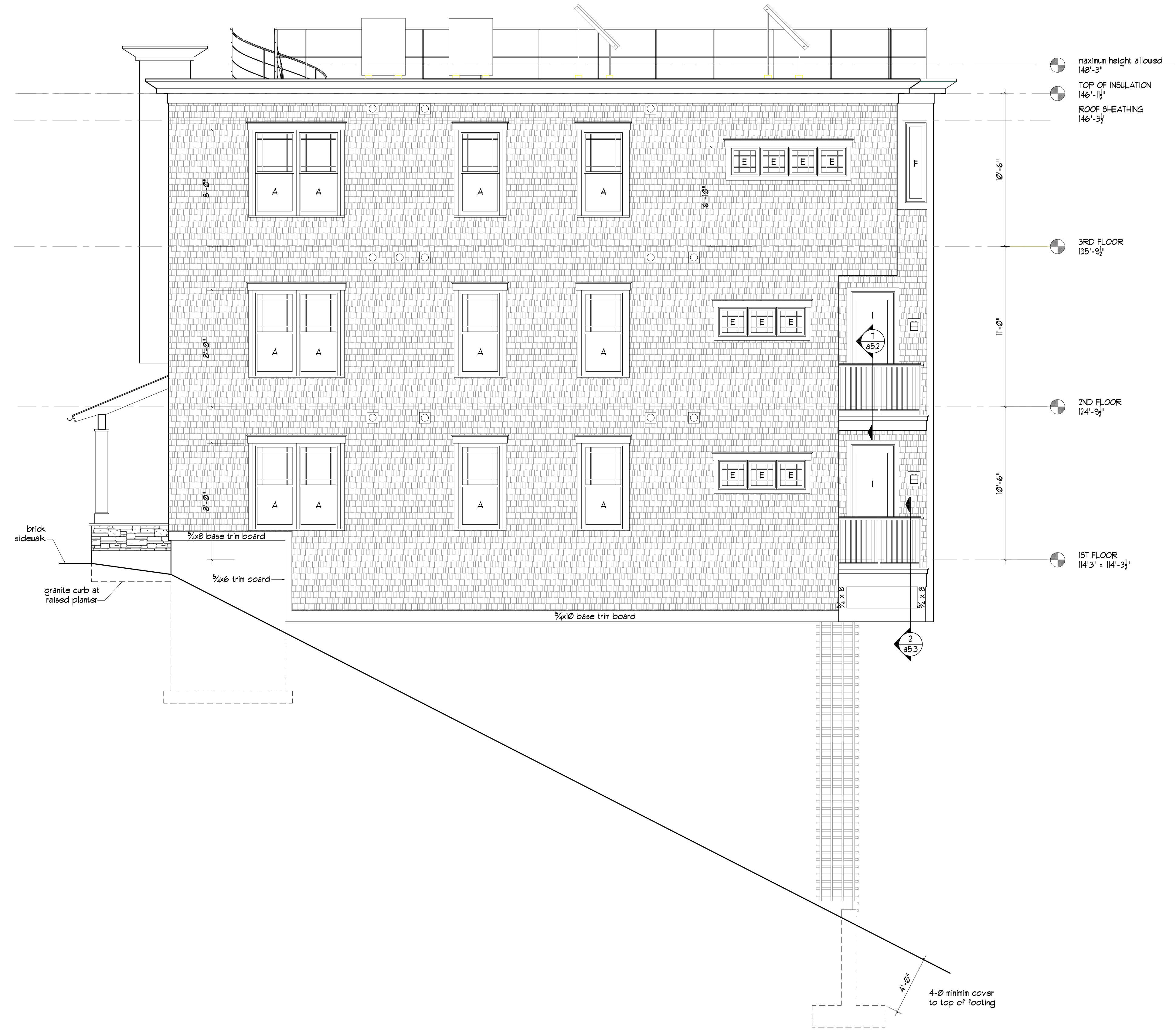
1 West Elevation 1/4" = 1'-0"
