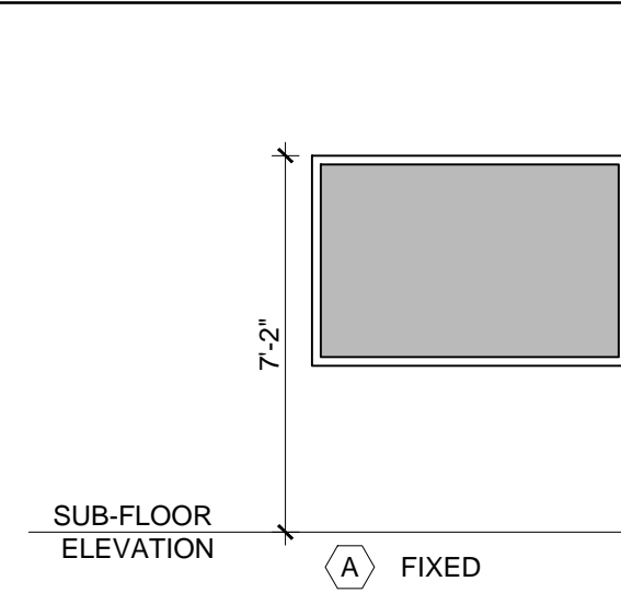
1 WINDOW TYPES 1/4" = 1'-0"
