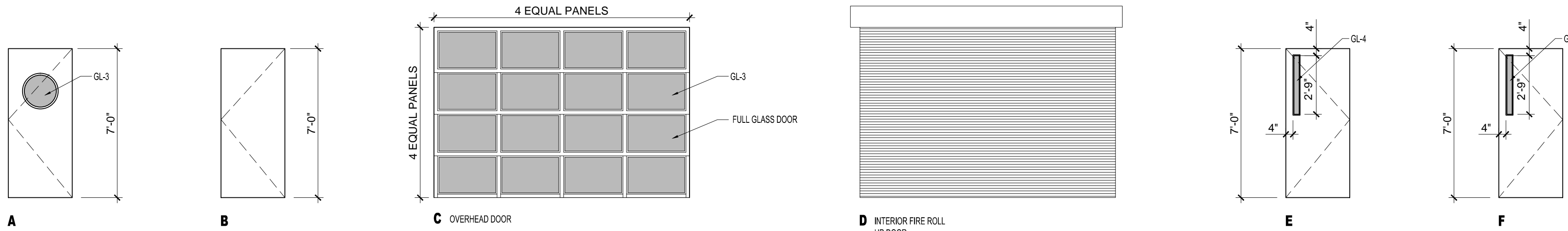
1 DOOR TYPES 1/4" = 1'-0"
