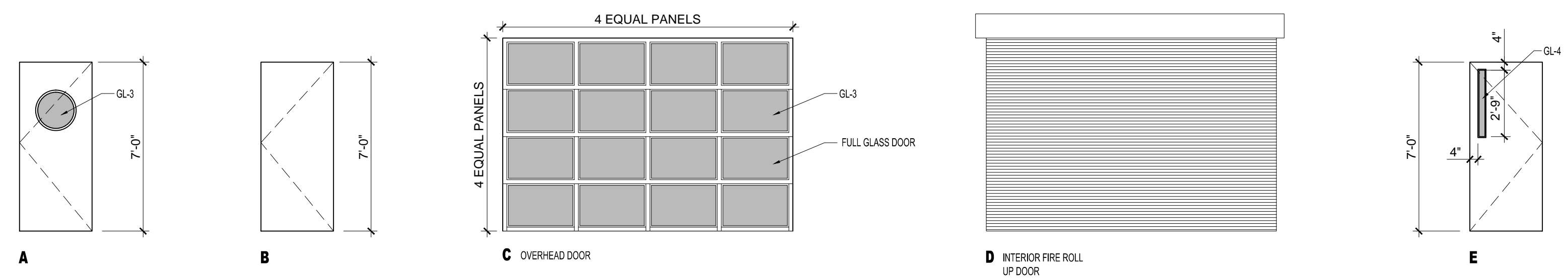
1 DOOR TYPES 1/4" = 1'-0"
