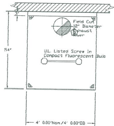
PLAN VIEW - Hood #1 4' 0.00" LONG 5424ND-2
