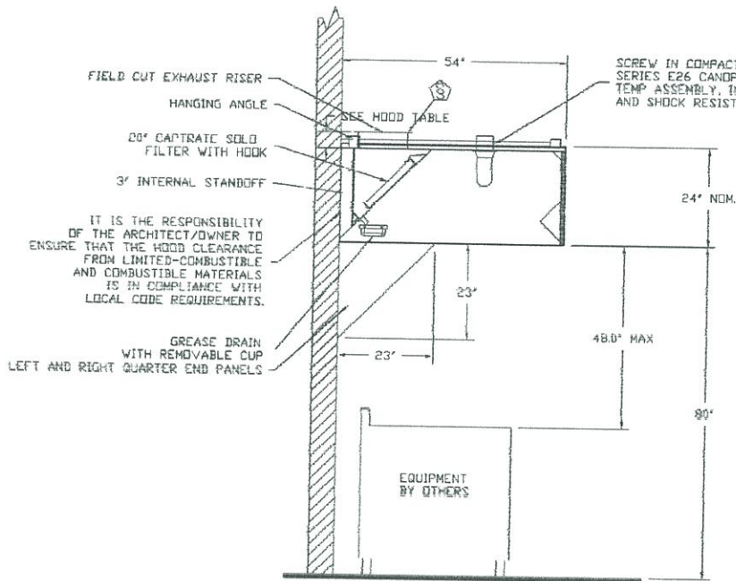
SECTION VIEW - MODEL 5424ND-2 HOOD - #1
