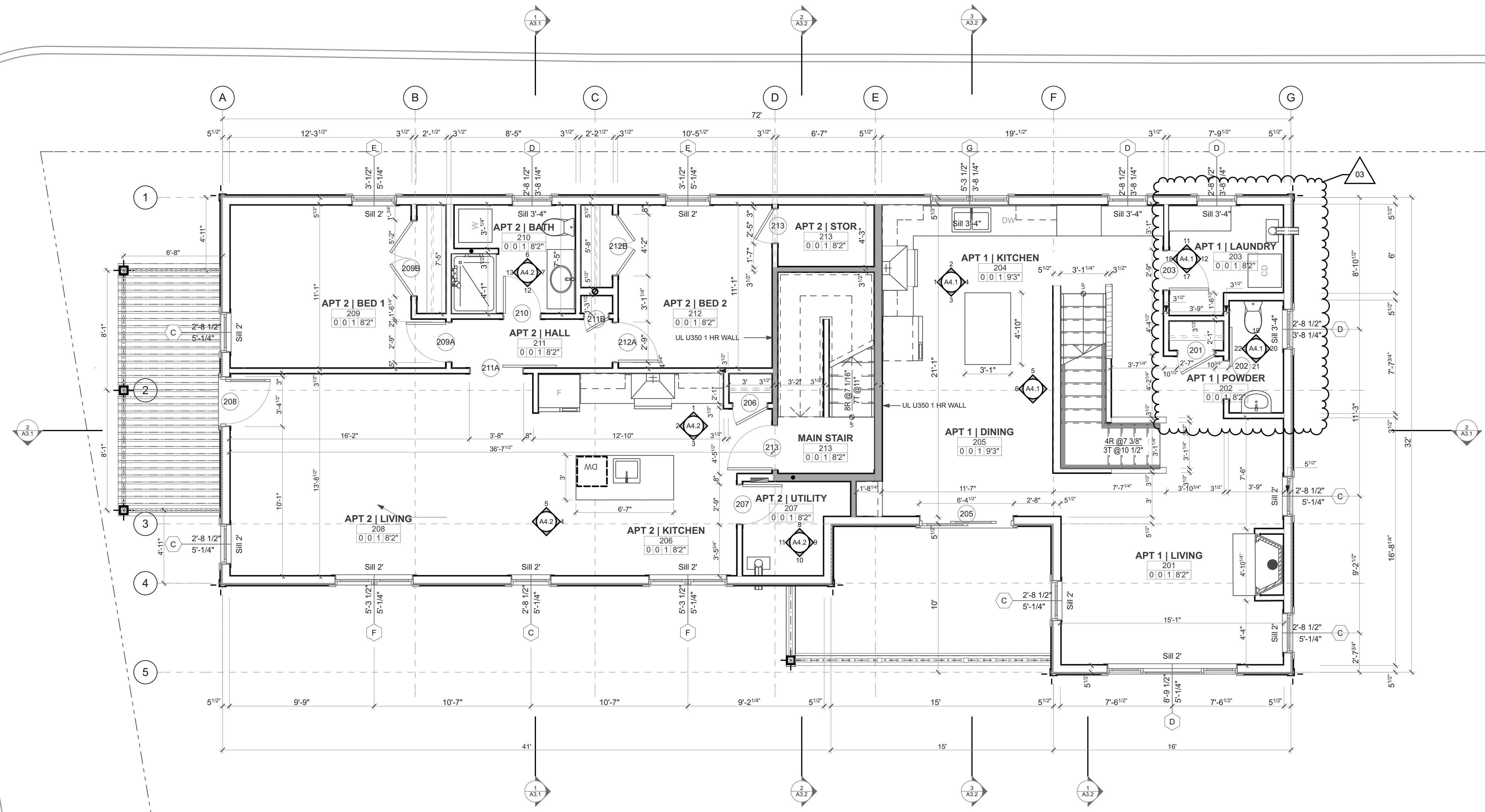
3 SECOND FLOOR A1.2 SCALE: 1/4" = 1'-0"
