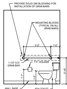
2 BATHROOM 106 - INTERIOR ELEVATIONS 1/8" = 1'-0"
