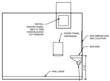
1 BATHROOM 107 - INTERIOR ELEVATIONS 1/8" = 1'-0"
