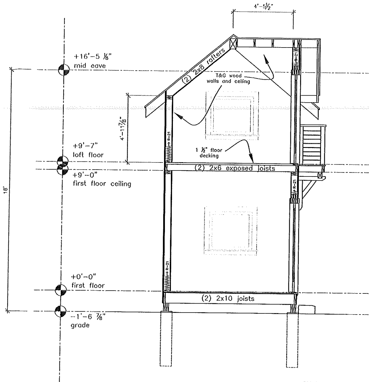
Ⓐ Cross Section 1/4" = 1'-0"
